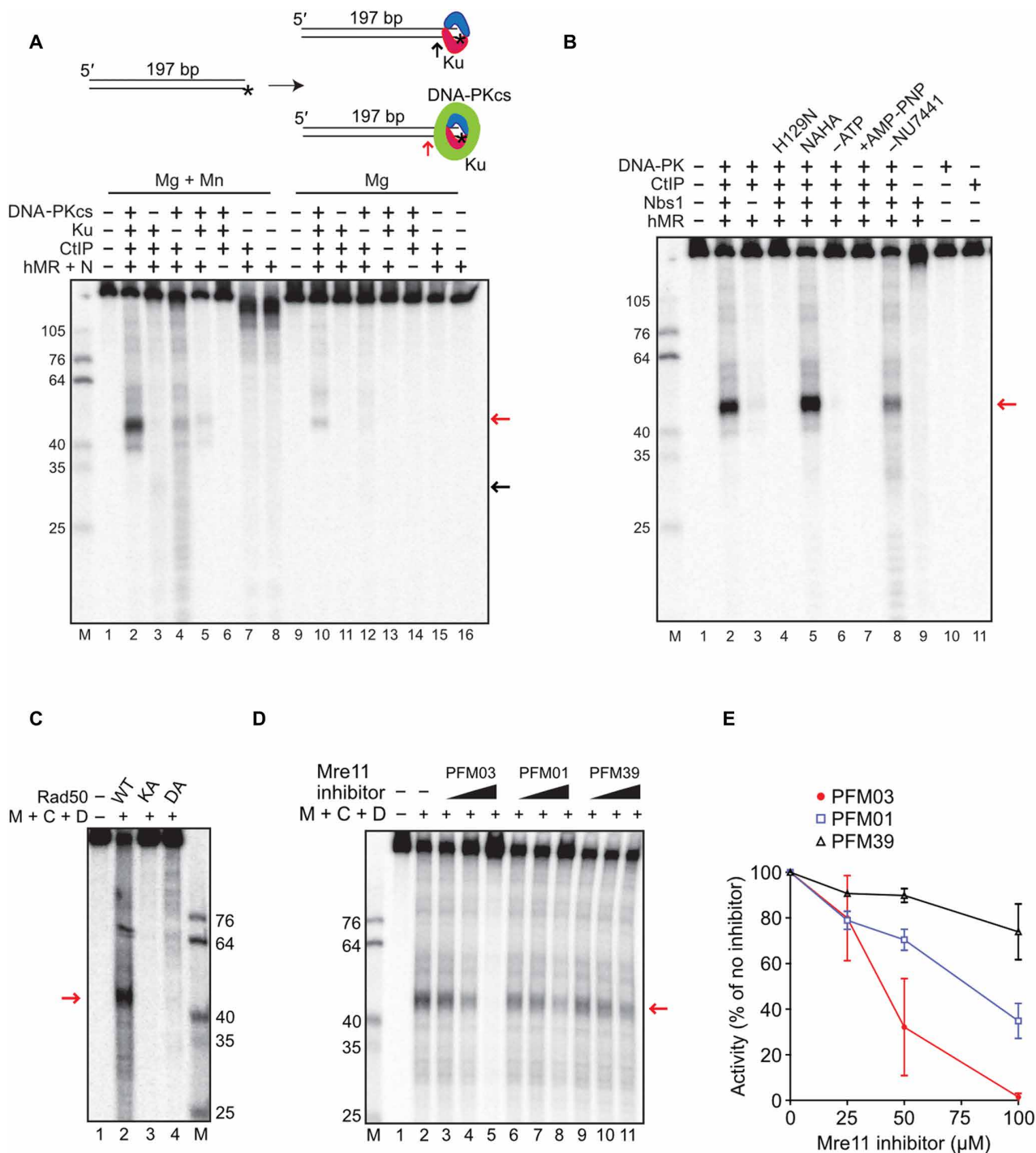
Fig. 1. Nucleolytic removal of DNA-PK by MRN and its stimulation by CtIP. (A) Nuclease reactions were performed with a 197-bp DNA substrate, 5' labeled with ^{32}\text{P} (asterisk), with MRN (50 nM), CtIP (80 nM), Ku (10 nM), and DNA-PKcs (10 nM) as indicated, in the presence of both magnesium and manganese (lanes 1 to 8) or magnesium only (lanes 9 to 16). All reactions contained the DNA-PKcs inhibitor NU7441. Products were visualized by denaturing PAGE and visualized by phosphorimager. Red and black arrows indicate the predominant product in the presence of DNA-PKcs and Ku, or Ku alone, respectively. (B) Nuclease assays were performed as in (A) in the presence of both magnesium and manganese with wild-type MRN or MRN containing nuclease-deficient Mre11 (H129N). Reactions without ATP or with AMP-PNP instead of ATP are indicated, as is the reaction without NU7441. (C) Nuclease assays were performed as in (A) in the presence of magnesium, manganese, ATP, NU7441, CtIP (C), and DNA-PK (D) with MRN (M) containing wild-type Rad50 (WT) or adenosine triphosphatase (ATPase)-deficient Rad50 K42A (KA) or D1231A (DA). (D) Nuclease assays were performed as in (A) in the presence of both magnesium and manganese with wild-type MRN in the presence of 25, 50, and 100 \mu\text{M} Mre11 inhibitors and NU7441. (E) Quantitation of the MRN endonuclease observed in the presence of Mre11 inhibitors expressed as percentage of the activity in the absence of inhibitors. Error bars represent SD from two replicates.
