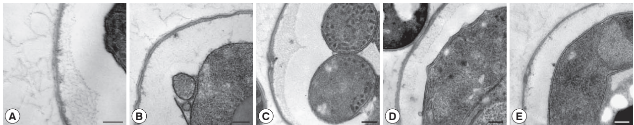
Fig. 3. Changes in the oocyst wall of C. parvum following gamma irradiation. (A) nonirradiated control; (B) 1 kGy; (C) 5 kGy; (D) 10 kGy; (E) 25 kGy. Bar=0.2 \mu m.
