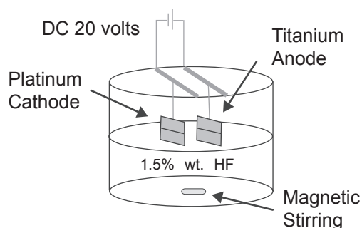
Figure 1 Schematic of the anodization system.
