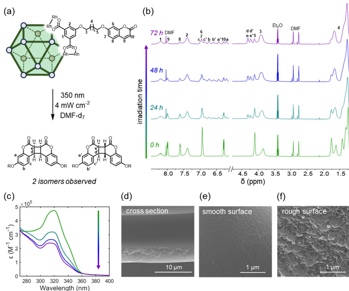
Fig. 3 (a) Irradiation of C 10 -Coumarin-RhMOPs at 350 nm results in the dimerization of their side chains. (b) 1 H NMR spectra of a 5 mM DMF-d 7 solution of C 10 -Coumarin-RhMOP after irradiation at 350 nm for 0 h (green), 24 h (teal), 48 h (blue), and 72 h (purple) reveal the emergence two correlated sets of aromatic and alkyl signals, suggesting the formation of two coumarin dimer isomers. Note that the absolute stereochemical configurations of the dimer isomers corresponding to each set of correlated peaks cannot be verified by this technique, and are therefore assigned arbitrarily. (c) UV-Vis spectra of the MOP solution at each irradiation time point reveal a decrease in the coumarin \pi \rightarrow \pi^* peak at 320 nm, corroborating the formation of cyclobutane dimers. (d–f) SEM images of the (d) cross section, (e) smooth surface, and (f) rough surface of a photopolymerized C 10 -Coumarin-RhMOP thin film produced via 350 nm irradiation of a 20 mM DMF solution of the cage.
