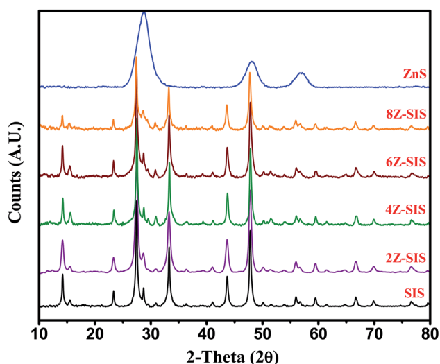
Fig. 1 XRD pattern for \text{SnIn}_4\text{S}_8 NPs, ZnS NPs and ZnS/ \text{SnIn}_4\text{S}_8 nanoheterostructure with different Z/S molar ratios.
