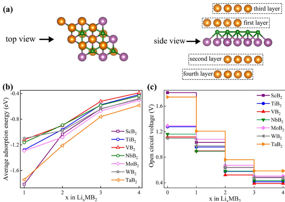
Fig. 5 (a) The structural configuration of four layers of Li atoms adsorbed on the surface of \text{MB}_2 ; (b) the change in average adsorption energy and (c) the open circuit voltage of \text{Li}_x \text{MB}_2 ( M = \text{Sc, Ti, V, Nb, Mo, W} and \text{Ta} ) as a function of Li concentration.
