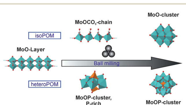
Fig. 5 Formation scheme for the mechanochemical synthesis of POMs.
