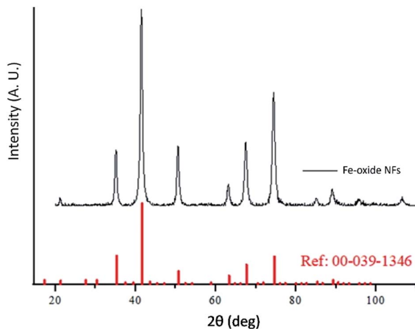
Fig. 4 XRD measurement for maghemite NFs and corresponding peak positions of the relevant JCPDS pattern for \gamma -Fe 2 O 3 .
