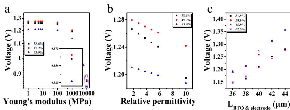
Figure 4. The open circuit voltage of the PENG at different polymer Young's modulus (a), permittivity (b), and the distance between electrode and BaTiO 3 cubes (c).
