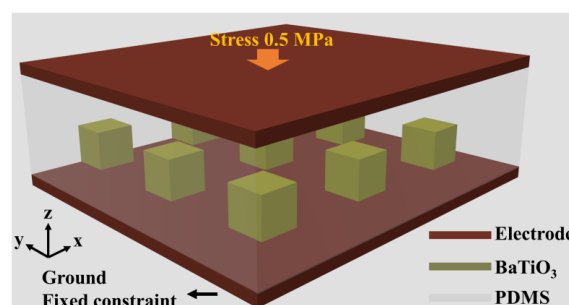
Figure 1. Schematic illustration of the BaTiO 3 /polydimethylsiloxane (PDMS) composite piezoelectric nanogenerator (PENG).
