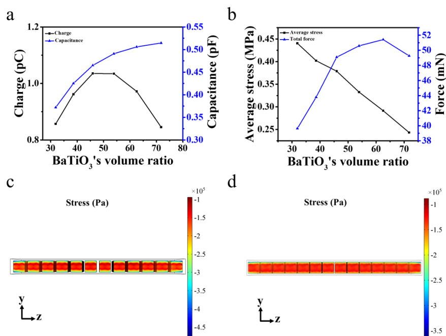
Figure 3. (a) The PENG's top surface charge and capacitance with different BaTiO 3 ratios. (b) The averaged stress and total force on the top surface of the embedded BaTiO 3 cubes. The distribution of stress in the BaTiO 3 at 45.9% (c) and 62.5% (d).
