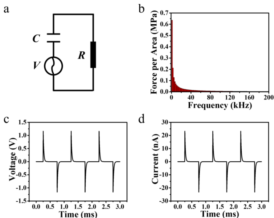
Figure 5. (a) The equivalent circuit of the composite PENG. (b) The spectral analysis of the square wave force. The output voltage (c) and current (d) at an external load with a resistance of 50 MΩ.
