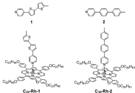
Fig. 2 Molecular structures of 1, 2, C 22 -Rh-1, and C 30 -Rh-2.
