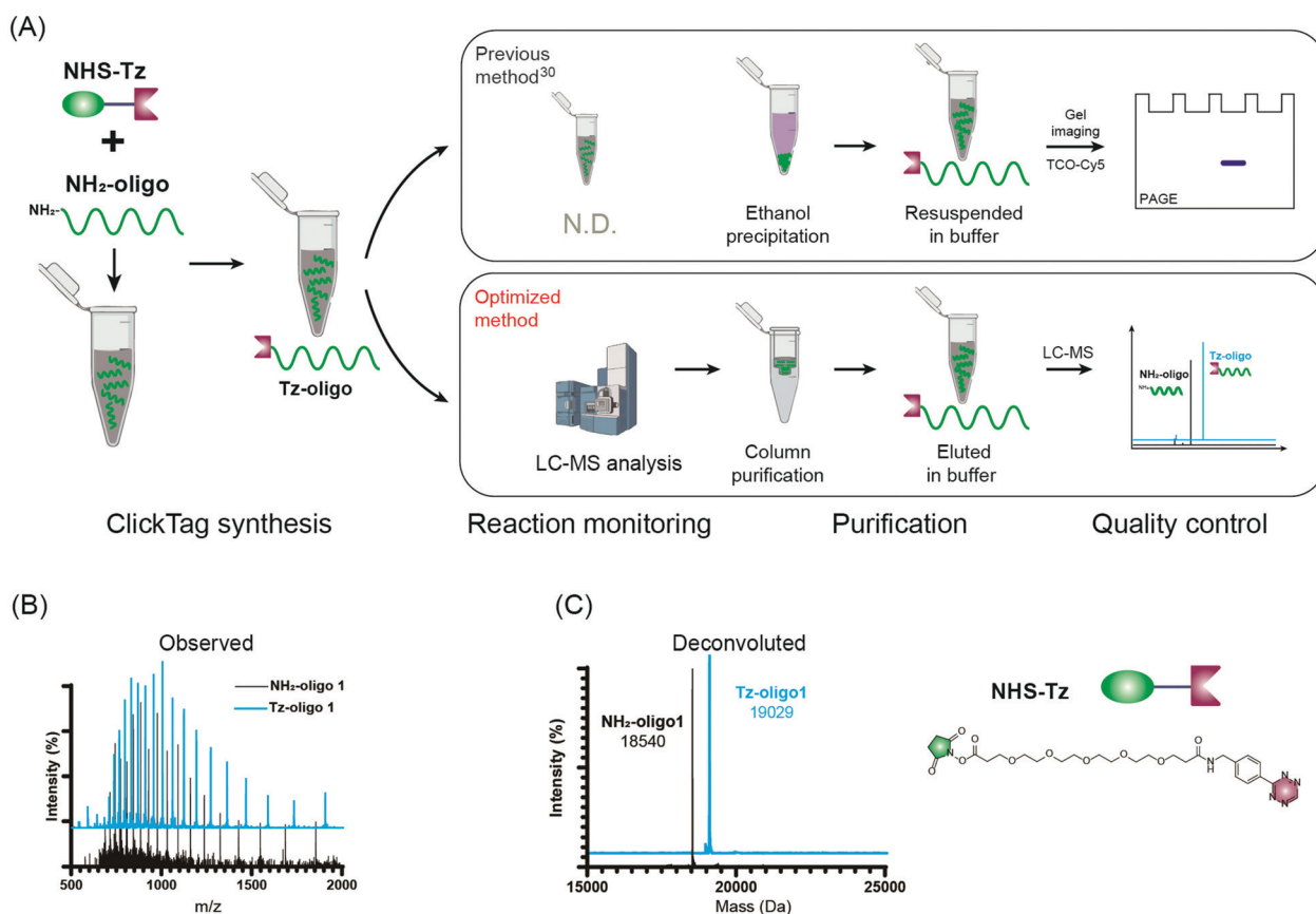
Fig. 1 The optimized synthesis procedure for Tz-oligos. (A) Schematic procedures of ClickTag synthesis. Previous method: top; optimized method: bottom. Observed (B) and deconvoluted (C) mass spectra of NH 2 -oligo 1 and final product Tz-oligo 1 (related to ClickTag1).
