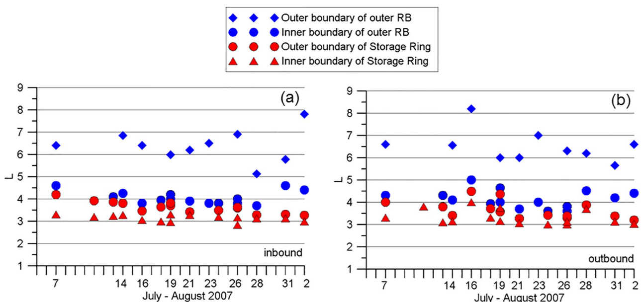
Figure 11. L-values for radiation belt boundaries determined from the background counts from (a) inbound and (b) outbound passes of both Cluster and Double Star satellites during the July–August 2007 event.
