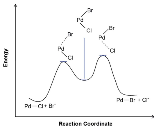
Scheme 3 Proposed reaction profile for the halide exchange reaction; [\text{Cl}]^+ + \text{Br}^- \rightarrow [\text{Br}]^+ + \text{Cl}^- . The transition state is proposed to have more Pd \cdots Cl bond dissociation character.
