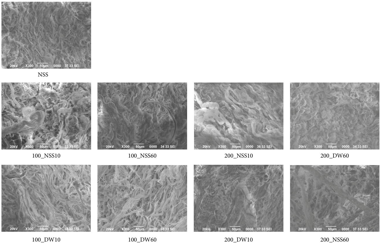
FIGURE 9: The SEM micrographs of pressurized skin. The SEM micrographs of the dermis in NSS, 100_NSS10, 100_NSS60, 200_NSS10, 200_NSS60, 100_DW10, 100_DW60, 200_DW10, and 200_DW60 are shown. The arrangement and proportion of collagen fibers were close enough and not adversely affected after pressurization, regardless of the processing time. Scale bar: 50 \mu m.
