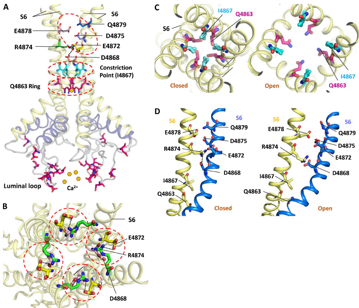
Figure 2. Structure of the RyR2 channel pore. (A) Detailed structure of the channel pore of RyR2, illustrating the major structural elements potentially involved in \text{Ca}^{2+} activation. (B) Top view of the channel pore, showing salt bridges potentially formed between D4868, E4872, and R4874. (C) Top view of the channel pore in a closed (left) and open (right) conformation. In the closed state, the constriction point (the narrowest part of the pore) is formed by I4867; when the channel opens, the constriction point shifts to Q4863. (D) Side chain orientation of critical residues in the S6 helices from neighboring subunits. The salt bridge between R4874 and E4872 is disrupted when the channel opens.
