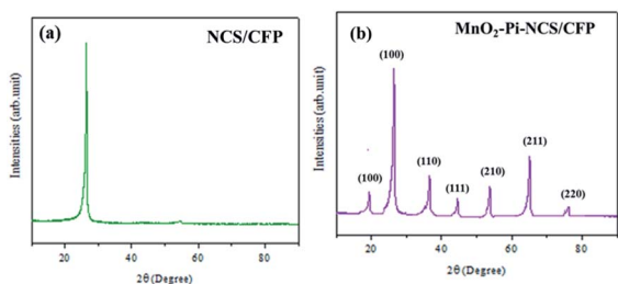
Fig. 4 XRD graphs obtained for (a) NCS/CFP and (b) MnO 2 -Pi-NCS/CFP electrodes.
