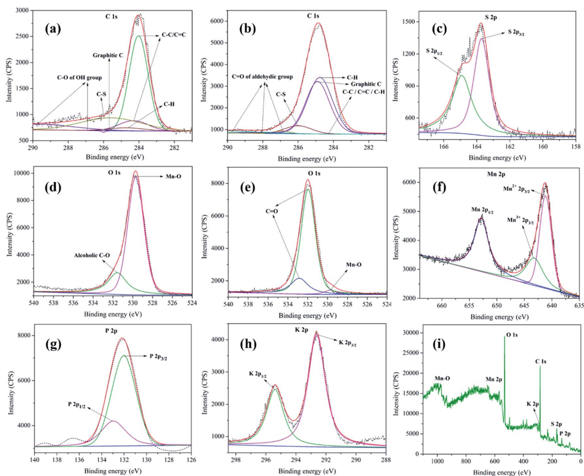
Fig. 5 XPS analysis of MnO 2 -Pi-NCS/CFP electrodes, showing C 1s spectrum (a) before and (b) after oxidation of thiophene methanol; (c) S 2p core level spectrum; O 1s spectra (d) before and (e) after oxidation; (f), (g) and (h) represent core level spectrum of Mn 2p, P 2p, and K 2p, respectively. (i) Wide XPS spectrum of MnO 2 -Pi-NCS/CFP electrode. The original spectra are indicated by dotted lines; the sum of deconvoluted peaks is represented by solid red lines.
