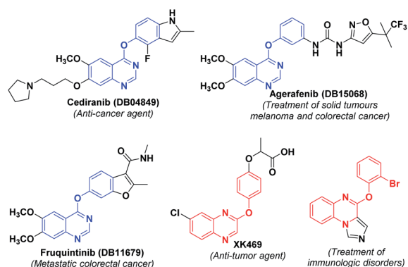
Fig. 1 Representative biologically active quinazolines and quinoxalines.
