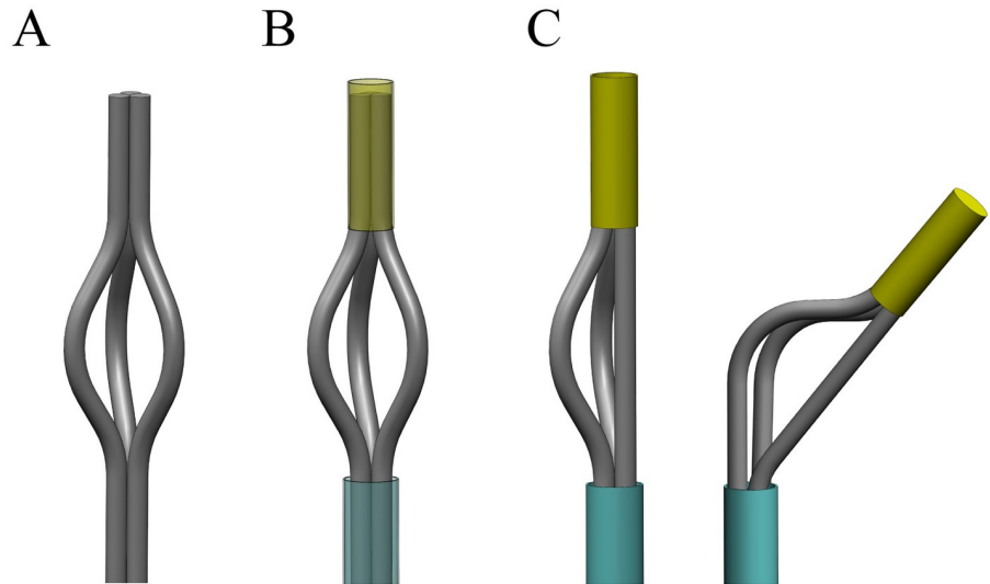
Fig 1. Schematic of the design of the probe tip. (A) Three elements with a pre-curve close to the tip. (B) The elements are connected at the tip and kept together along the body with a tubular sheath. (C) The element pulled is straightened and helps the other two pre-curved elements to bend, bringing the tip in a bent position.
