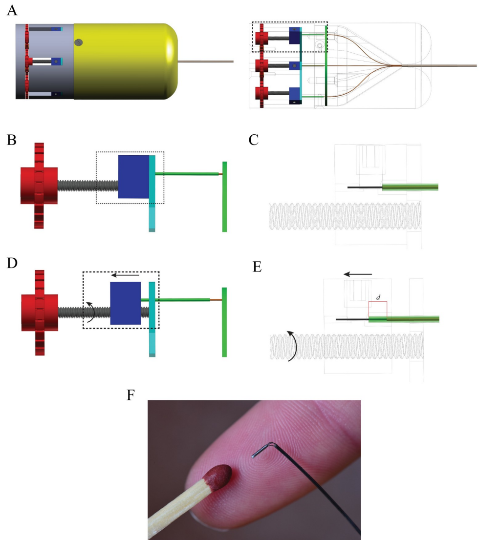
Fig 3. Actuation mechanism of the probe prototype. (A) 3D drawing of the actuation unit (left) and the leadscrew mechanisms with the wires visible inside the main body (right). (B) Close-up of one leadscrew mechanism at the initial position. (C) Close-up of the wire clamped inside the block surrounded by the Nitinol tube (orange) and the rigid tube (green), which is glued inside the block. (D) Close-up of one leadscrew mechanism after the wheel has been turned and the block with the wires clamped inside translated. (E) Close-up showing the position of the wire, Nitinol tube, and rigid tube after the block translation. When the block translates, the wire is retracted leaving behind the Nitinol tube that is glued to the ring-shaped object (green). The rigid tube protects the length of the wire d that is not supported by the Nitinol tube. (F) Photograph of the tip bent after retraction of one wire. Dashed rectangular windows highlight the areas of interest. Arrows show the directions of motion of the parts.
