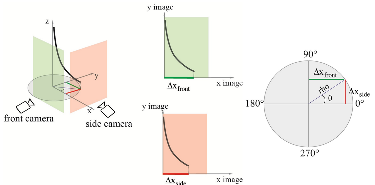
Fig 9. Schematic representation of the probe on the 3D plane. In red, the y-coordinate of the final point of the probe ( \Delta x_{side} ). In green, the x-coordinate of the final point of the probe ( \Delta x_{front} ). The angle \theta is equal to \arctan(\Delta x_{side}[\text{mm}], \Delta x_{front}[\text{mm}]) , and the distance \rho is
