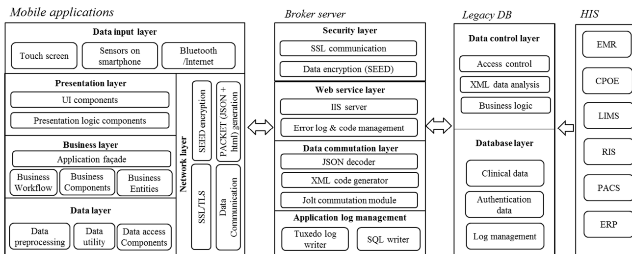
Figure 5. Technical architecture of mobile sensor applications. JSON: JavaScript Object Notation, SSL: Secure Socket Layer, TLS: Transport Layer Security, IIS: Internet Information Services, HIS: Hospital Information System, EMR: Electronic Medical Record, CPOE: Computerized Physician Order Entry, LIMS: Laboratory Information Management System, RIS: Radiology Information System, PACS: Picture Archiving Communication System, ERP: Enterprise Resource Planning.
