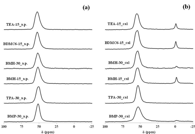
Fig. 6 27 Al MAS NMR spectra of the as-prepared (a) and calcined (b) ZSM-5 and beta zeolites.
