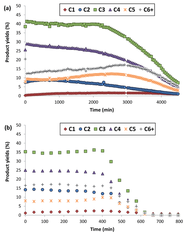
Fig. 9 Product yields obtained using BMP-30 (a) and TPA-30 (b) as catalysts for the MTO reaction (conditions: T = 450\text{ }^{\circ}\text{C} , \text{WHSV} = 10\text{ h}^{-1} , W_{\text{cat}} = 50\text{ mg} ).
