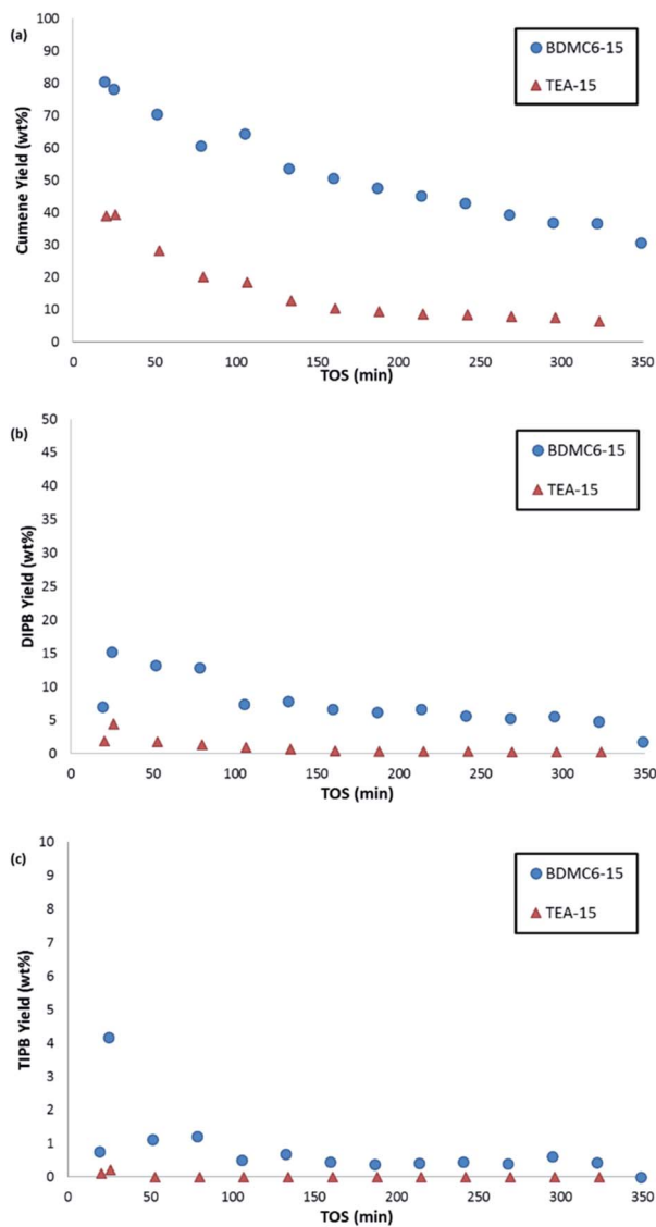
Fig. 12 Selectivity to cumene (a), di-isopropylbenzene (b), and tri-isopropylbenzene (c) with TOS for the liquid phase alkylation of benzene with propylene using nanosized betas as catalysts.
