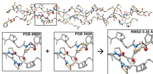
Fig. 3 Aza-proline mimics proline in backbone of CMP. (Top) Superposition of crystal structures of CMPs 1 and 2 showing close matching of backbone and side chain conformations throughout; RMSD = 0.36 Å. (Bottom) Close-up of boxed region in 1 (PDB 6M80), 2 (PDB 5K86), and overlay of the two structures, illustrating correspondence between conformation of azPro7 in 1 and Pro7 in 2 .
