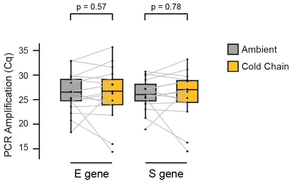
Fig. 2. Effect of shipping conditions on SARS-CoV-2 RNA stability in saliva samples. Comparison of Cq values (E gene and S gene) in paired saliva and/or NTS samples following shipment to the laboratory under room temperature (RT) or cold chain (CC) conditions. P values are for a 2 tailed Wilcoxon test.
