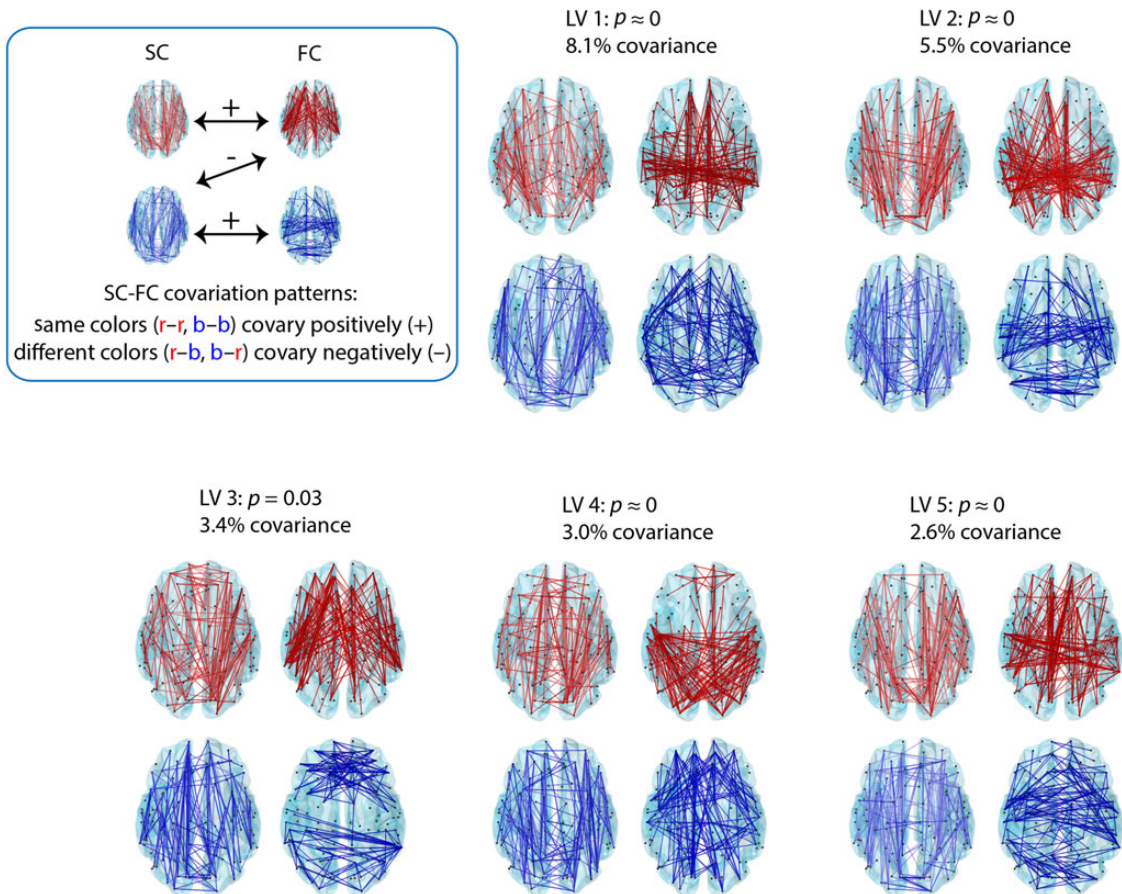
Figure 3. Spatial configuration of optimally covarying SC-FC networks. PLS analysis revealed 5 statistically significant SC-FC patterns. Statistical significance is assessed using permutation tests, and effect size is estimated from the magnitude of the singular value associated with each pattern (see Materials and Methods). Each LV is comprised of a weighted pattern of structural (left) and functional (right) connections. Bootstrap resampling is used to construct a 95% confidence interval for each connection weight; the top 5% most reliable connections are shown. Connections with positive weights are shown in red and connections with negative weights are shown in blue. SC-FC patterns with the same color covary positively with each other, while SC-FC with different colors covary negatively.
