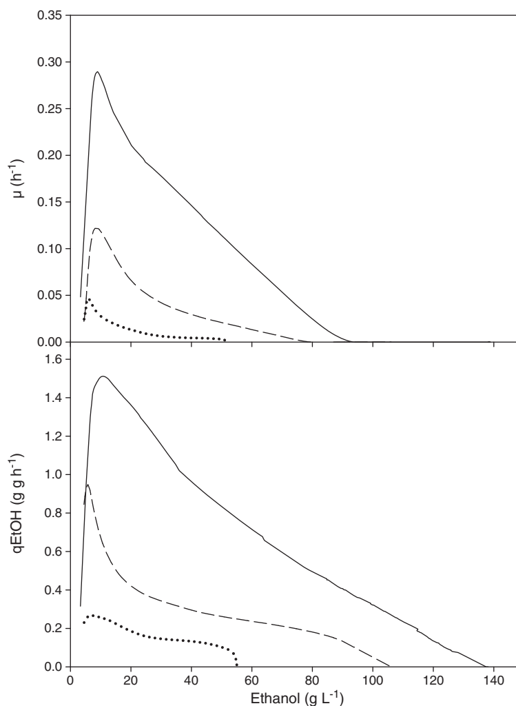
Figure 2 Specific growth rate ( \mu ) and specific ethanol production rate ( q_{\text{EtOH}} ) as functions of ethanol concentration. Strains: wild type CENPK113-7D (—), TEFmut7 (---), TEFmut2 (.....).
