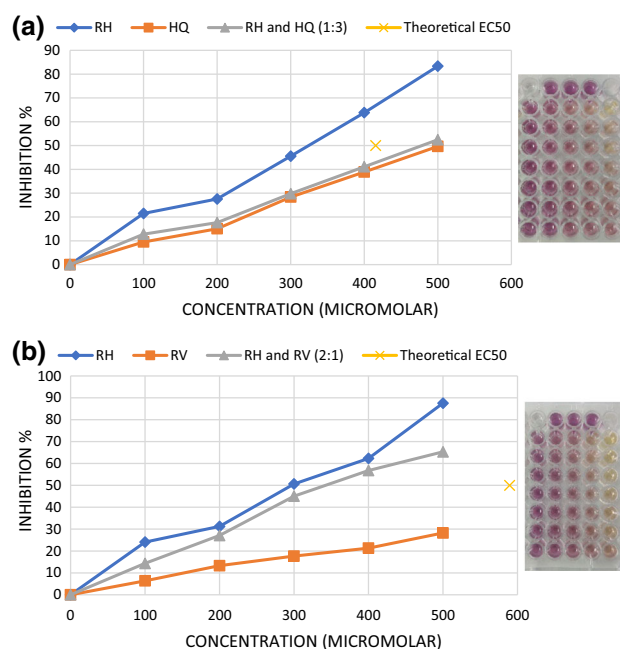
Fig. 4 a Antagonistic antioxidant interaction between rutin hydrate and hydroquinone in 1:3 ratio b Synergistic antioxidant interaction between Rutin hydrate and Resveratrol in 2:1 ratio. Theoretical EC 50 is calculated by mixing the individual graphs of both compounds. Theoretical EC 50 value less than the experimental value shows antagonism, whereas theoretical EC 50 value more than the experimental value shows synergism. Inset represents a photo of 96 well plate
