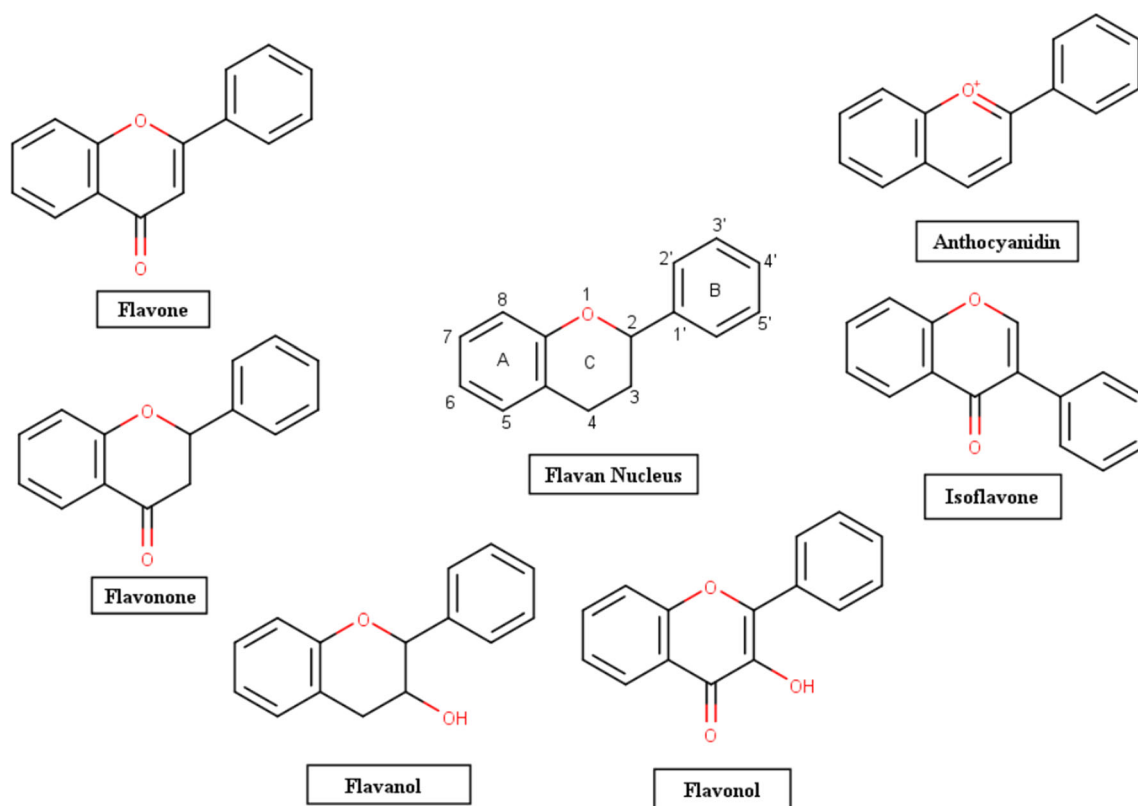
Fig. 1 Basic flavan structure and chemical structures of flavanoid subgroups. Structures are drawn using Marvin sketch software
