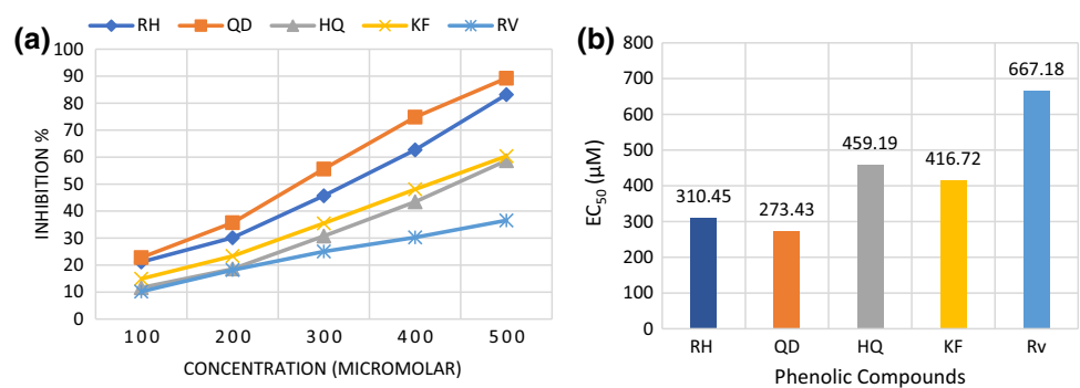
Fig. 2 a: DPPH radical scavenging activity (%) b: EC 50 values of selected flavonoid and non-flavonoid phenolic compounds. RH-Rutin hydrate; QD-Quercetin dihydrate; HQ-Hydroquinone; KF-Kaempferol; RV-Resveratrol
