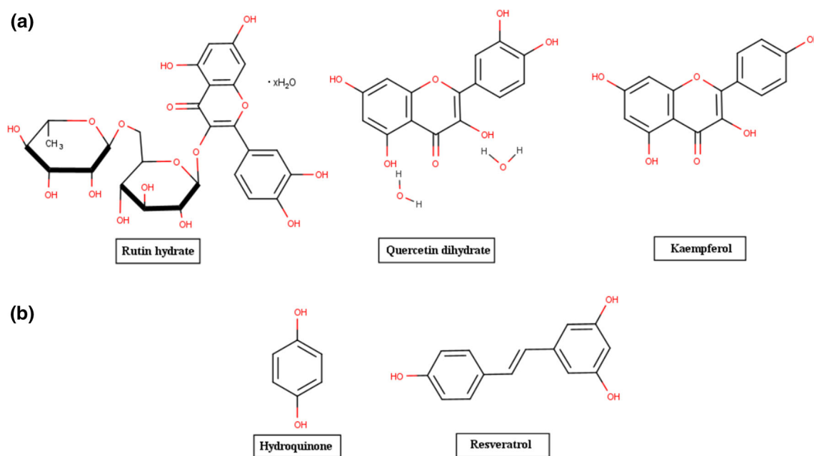
Fig. 3 Chemical structures of a Flavonoids, and b Non-flavonoid phenolic compounds. Structures are drawn using Marvin sketch software
