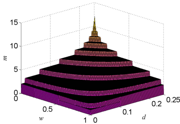
Figure 5. The number of distillation steps m needed for finally getting the aim state |W_3^{\varepsilon_0}\rangle .
