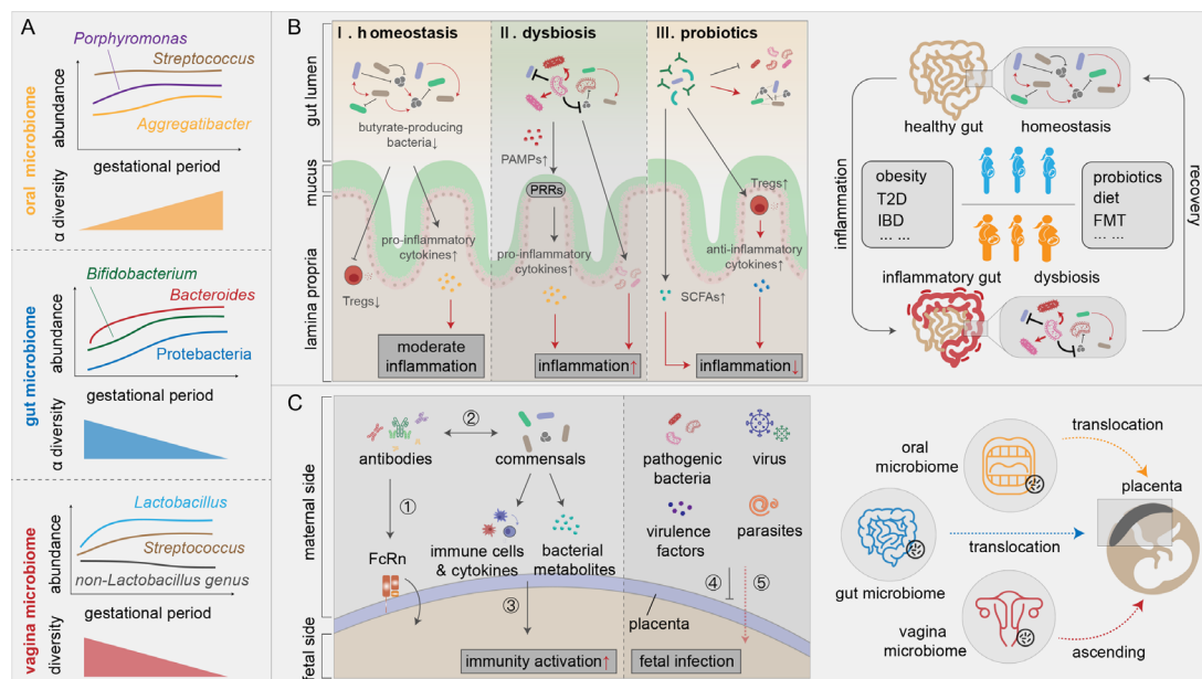
Figure 2 Microbial variation and transmission during pregnancy. (A) Variation in the abundance of representative bacteria in the maternal oral cavity, gut and vagina during pregnancy. (B) Host-microbe interaction in the maternal gut. Under healthy conditions, the gut microbiome and immune response of pregnant women is similar to that in individuals with metabolic syndromes, characterised by decreasing butyrate-producing bacteria and increasing proinflammatory cytokines, inducing moderate inflammation (I). When mothers have conditions such as T2D, obesity or IBD, deviation of the gut microbiome associated with alteration of the immune response is observed during pregnancy, increasing the risk of inflammatory diseases and gut leakage. Increased intestinal permeability allows the entry of bacterial toxins into the systemic circulation and induces multiple diseases (II and the left panel). Some interventions, such as probiotic, anti-inflammatory diet or FMT interventions, may restore dysbiosis of the gut microbiome and reduce inflammatory responses (III and the left panel). (C) Maternal-fetal interface communication during pregnancy. Maternal antibodies such as IgG are transferred to the fetus via FcRn (case 1). Some bacterial molecules are bound to maternal IgG and are transferred to the offspring (case 2). Such vertical transmission provides protection to the fetus. Fetal immune responses can also be activated by bacterial components or bacterial metabolites from mothers (case 3). Other substances, such as viruses, pathogenic bacteria, virulence factors and parasites that are harmful to the fetus are usually unable to cross the placenta (case 4, black lines with flat ends), except in situations of maternal infections (case 5, red dotted arrows). Translocation of the microbiome between maternal body sites (oral cavity, gut and vagina) and the fetus was observed. Whether the detection of microbes in the placenta is derived from contamination is highly debated, and thus, dotted lines are used for microbial translocation (the left panel). FcRn, neonatal Fc receptor; IBD, inflammatory bowel disease; PAMPs, pathogen-associated molecular patterns; PRRs, pattern recognition receptors; SCFAs, short-chain fatty acids; Tregs, regulatory T cells; T2D, type 2 diabetes.
