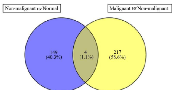
Fig. 1. Venn diagram of the differentially expressed genes obtained from non-malignant/normal and malignant/non-malignant analysis
