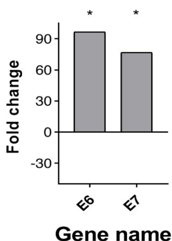
Fig. 4. Comparison of the fold changes of the viral onco-genes (E6 and E7) between the malignant CC patients and pre-malignant cases
