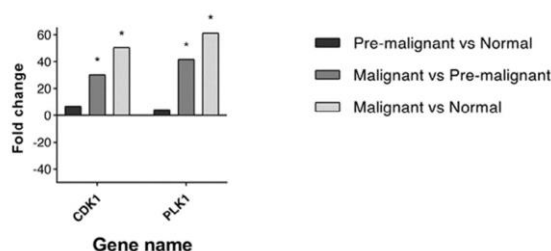
Fig. 3. Comparison of the fold changes of 2 identified hub genes (CDK1 and PLK1) using Real-Time PCR among patients with malignant cervical cancer, pre-malignant lesions and normal individual.
