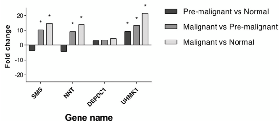
Fig. 2. Comparison of the fold changes of 4 identified common transcriptional signatures using Real-Time PCR among patients with malignant cervical cancer, and pre-malignant lesions and normal individuals
