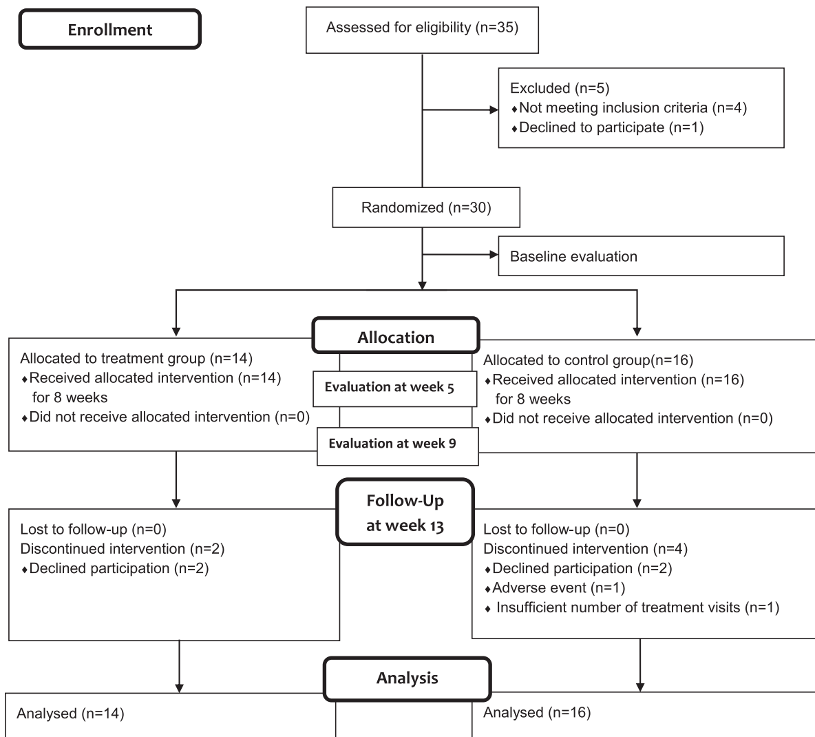
Fig. 1. Flow chart
