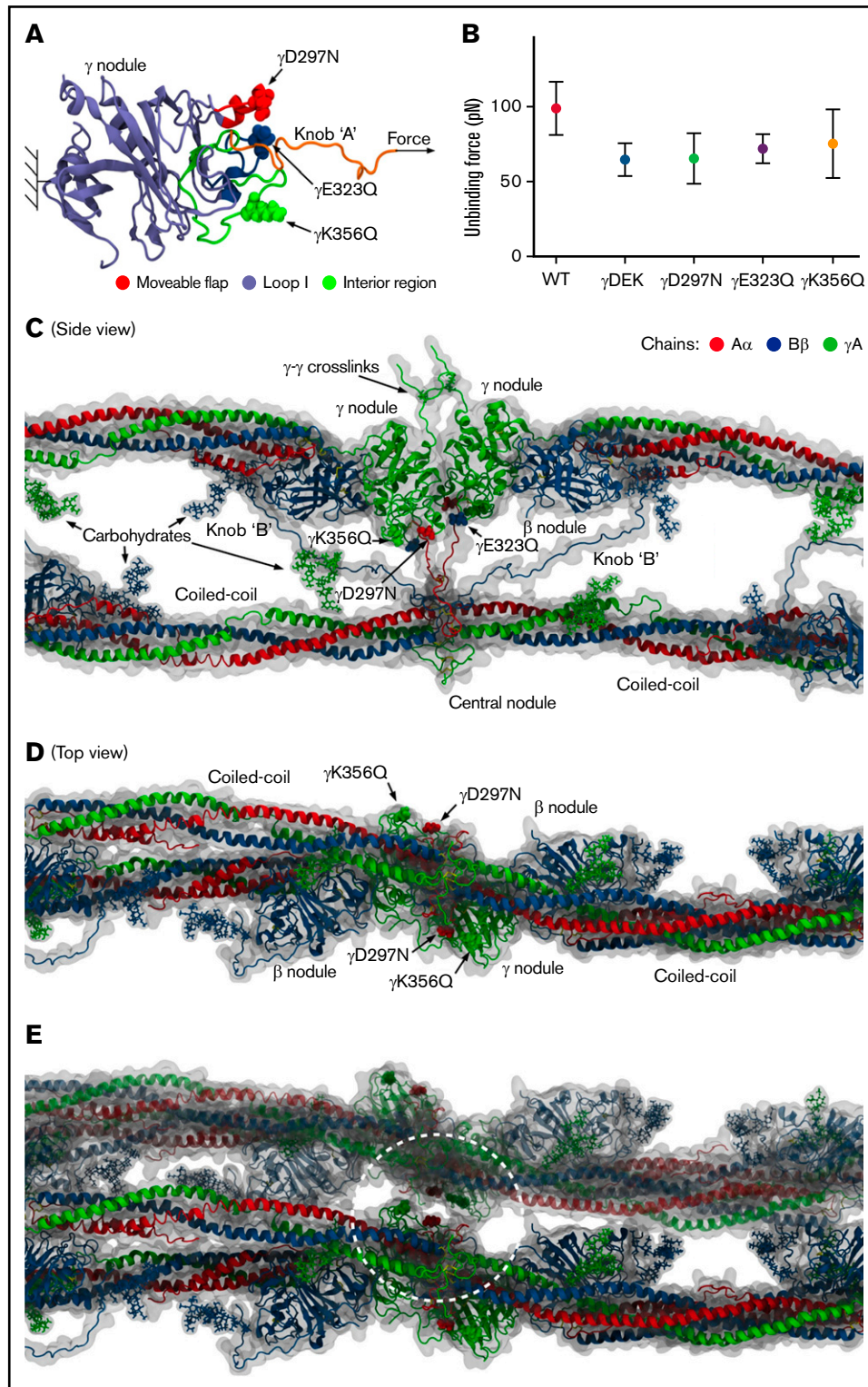
Figure 6. Computational molecular modeling. (A) Complete atomic structure of the A:a knob-hole complex (in ribbon representation), extracted from the structures of fibrin oligomers 6,36 at pH 7.0 and 25°C, showing hole a with the following binding determinants: the interior region (residues \gamma Trp335-Asn365; shown in green), loop I ( \gamma Trp315-Trp330; in blue), and movable flap ( \gamma Phe295-Thr305; in red) in the \gamma -nodule, and knob A (residues \alpha Gly17-Cys36; shown in orange). Also shown are the setup for the dynamic force experiments in silico, for example, the constrained residue \gamma Lys159 in the \gamma -nodule in hole a and tagged residue \alpha Cys36 in knob A, and the direction of pulling force (indicated by the arrow), and single-point mutations corresponding to variants \gamma D297N, \gamma E323Q, and \gamma K356Q (small arrows). (B) The average bond-rupture forces and SDs (mean \pm SD, N = 5 simulation runs) for WT and variants \gamma D297N, \gamma E323Q, \gamma K356Q, and \gamma DEK extracted from the simulations. (C-D) The side view
