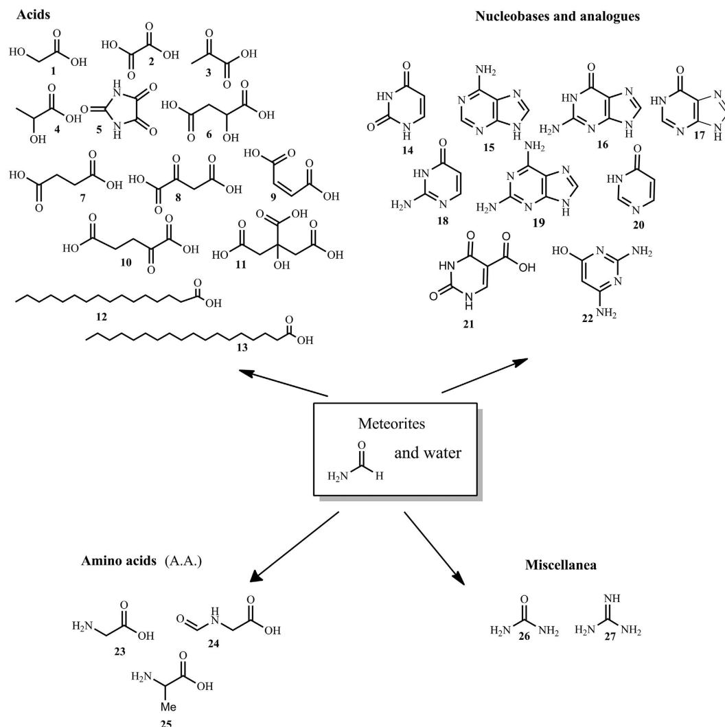
Figure 1. Prebiotic synthesis of biomolecules from meteorite and water in the presence of formamide.
