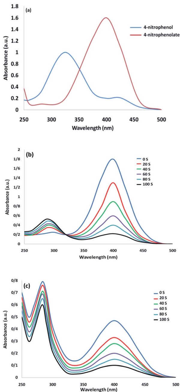
Fig. 7 UV-vis spectra of (a) 4-NP before and after adding the solution of \text{NaBH}_4 ; (b) the consecutive reduction of 4-NP to 4-AP; as well as (c) 2-NA to o -PDA on the \text{CoMn}_2\text{O}_4/\text{APTPOSS}@FPS NPs catalyst.
