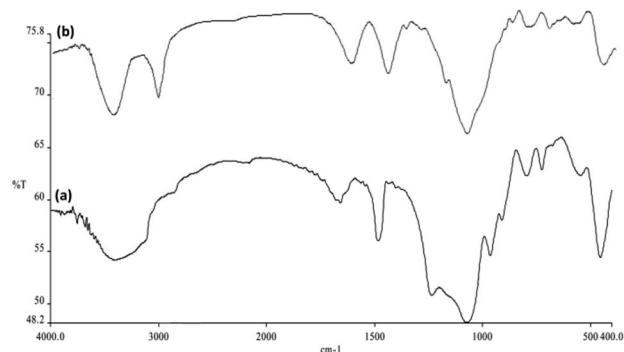
Fig. 6 Fourier transform infrared spectroscopy (FTIR) spectra of (a) FPS NPs, and (b) CoMn 2 O 4 /APTPOSS@FPS NPs.
