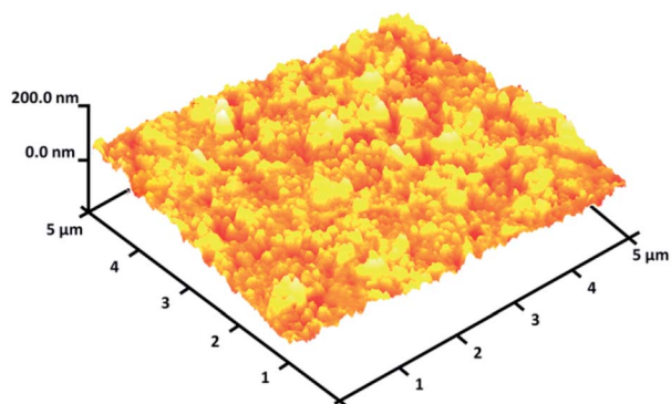
Fig. 4 Three-dimensional AFM images of the CoMn 2 O 4 /APTPOSS@FPS NPs.
