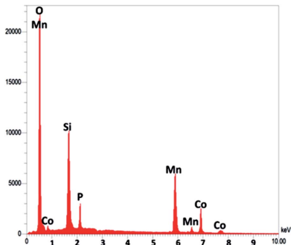
Fig. 3 EDX spectrum of CoMn 2 O 4 /APTPOSS@FPS.
