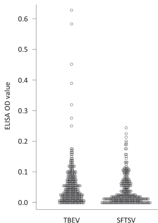
Fig. 2. Distribution of OD values obtained by IgG indirect ELISA. The dots indicate the OD values at 415 nm of IgG indirect ELISA for Tick-borne encephalitis virus (TBEV) and Severe fever with thrombocytopenia syndrome virus (SFTSV). OD: optical density. Means of OD value were obtained from duplicate experiments.
