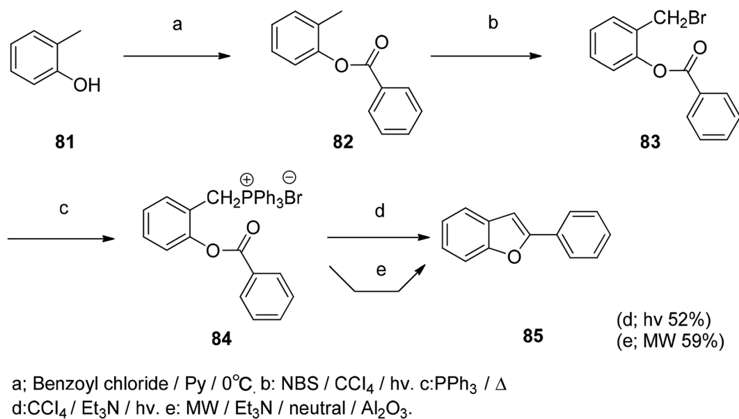
Scheme 4 The benzofuran compound was synthesized by the photochemical reaction method under both hν and MW conditions.
