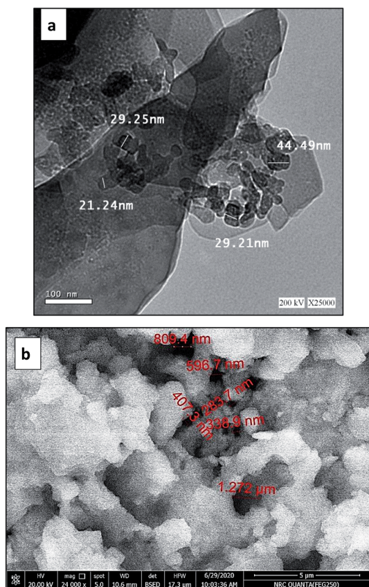
Fig. 2 (a) TEM image of ZnO nanoparticles, (b) SEM image of Pec/CS/ZnO nanocomposite.
