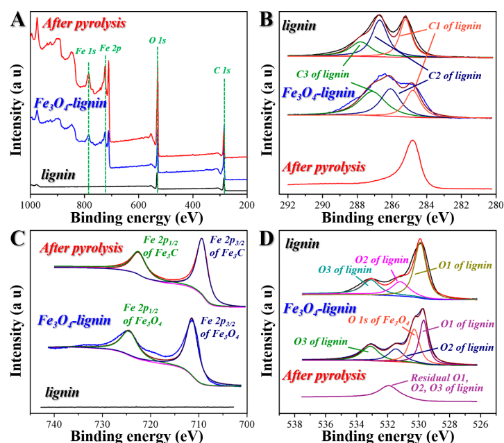
Figure 3. (A) X-ray photoelectron spectroscopy (XPS) spectra of lignin, \text{Fe}_3\text{O}_4 -lignin and the sample after pyrolysis process. (B–D) The corresponding high-resolution XPS spectra in C 1s, Fe 2p and O 1s, respectively.
