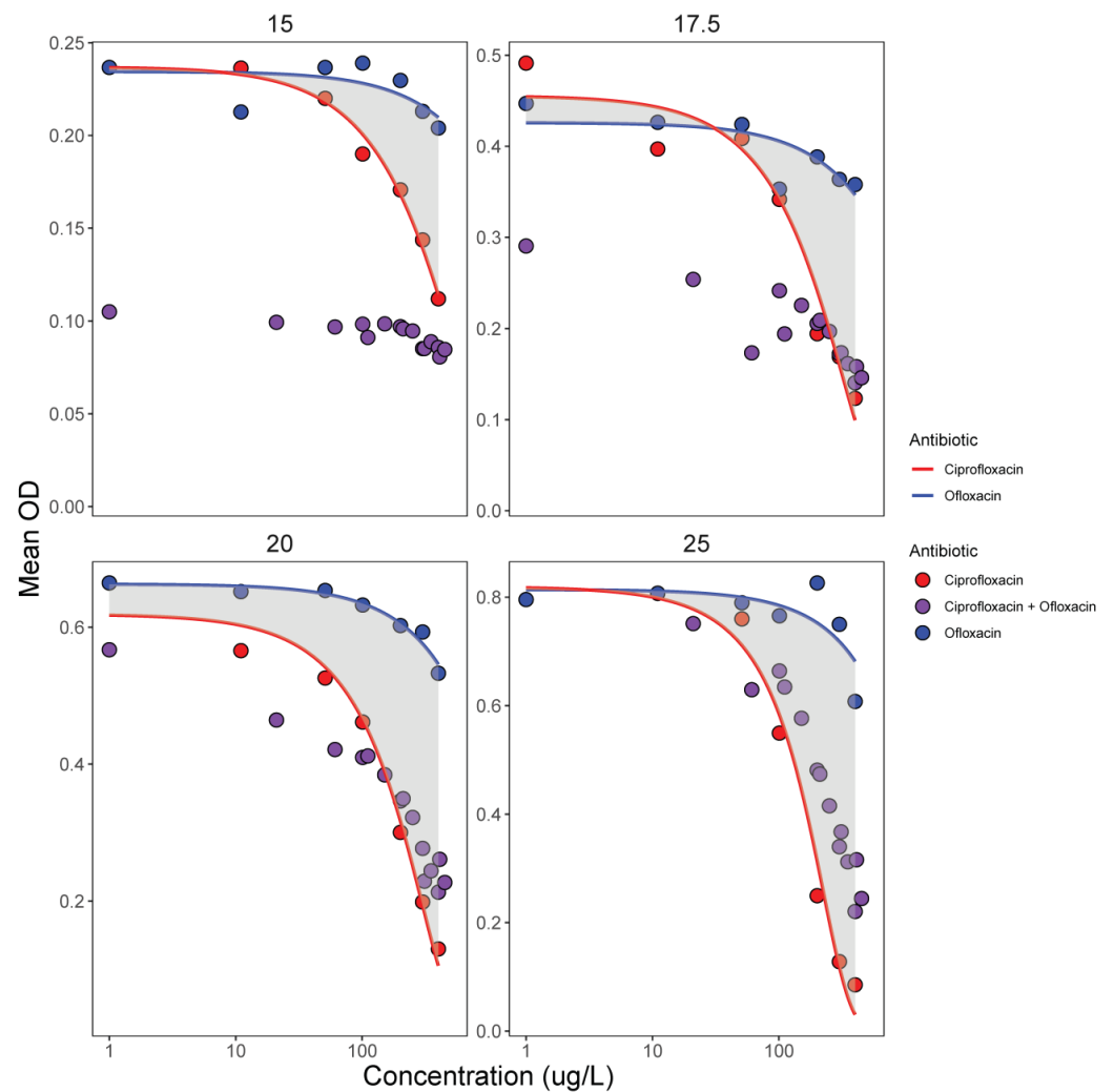
Figure 5. Potency of antibiotic mixtures of ciprofloxacin and ofloxacin (in 33 different proportions) compared to the dose–response of the single antibiotics (importantly, concentration range shown)
