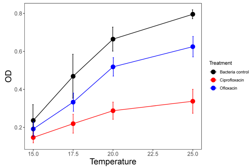
Figure 3. Optical density (means \pm SE) at four different temperatures averaged for microcosms with P. fluorescens only (control) and those that also contained a single antibiotic. The data shown for the antibiotic treatments are averaged across all concentration treatments from 10 to 500 \mu\text{g/L} .
