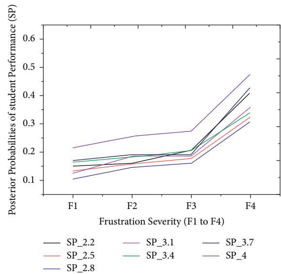
FIGURE 8: The probabilities of P2 are evolving with a change in frustration severity.
