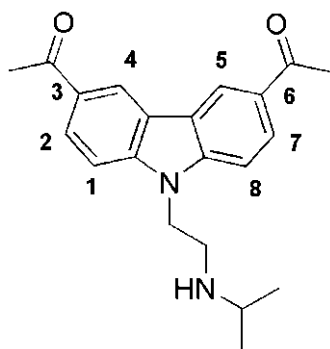
Figure 1. Structure of curaxin CBL0137.
