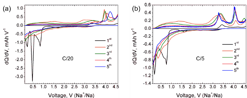
Figure 6. dQ/dV curves of \text{Na}_9\text{V}_{14}\text{O}_{35} in Na half-cell for the first five cycles at C/20 (a) and C/5 (b) current rates.
