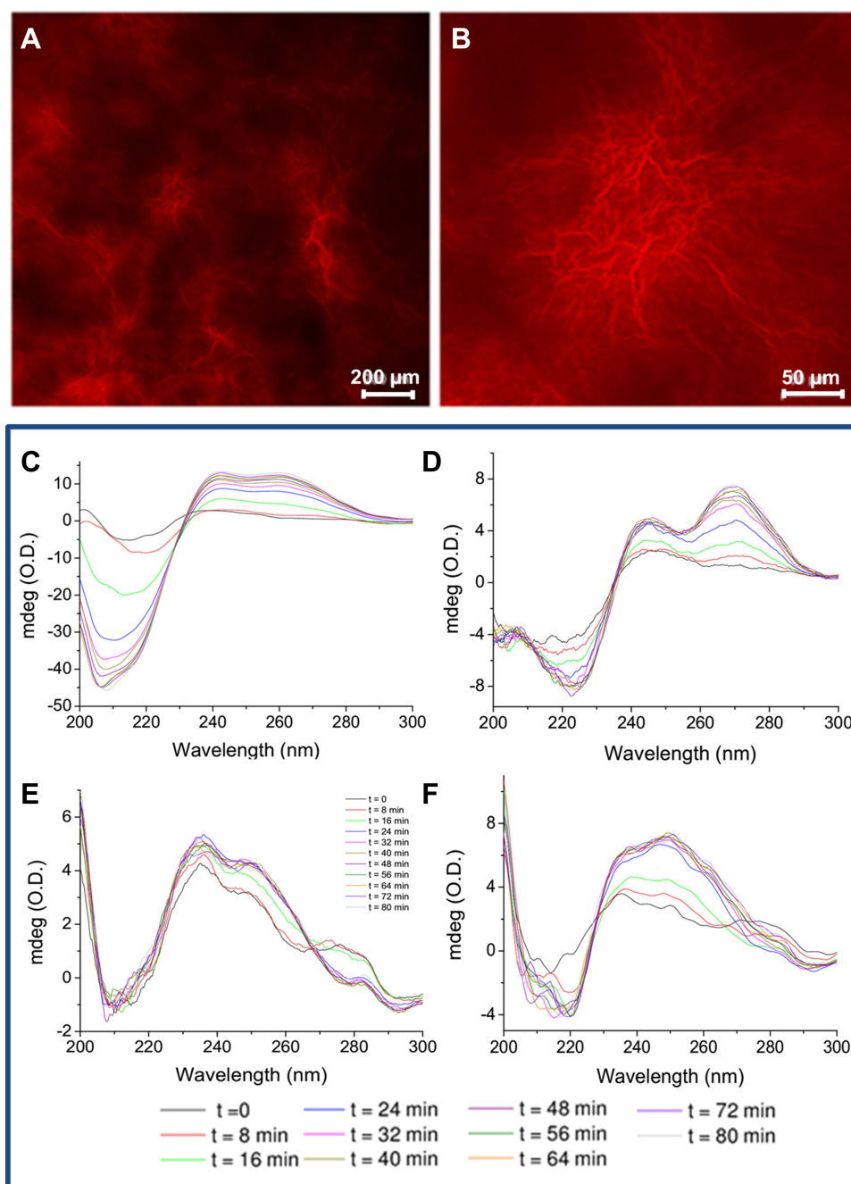
Figure 2 Characterization of mixed HGs. (A and B) Confocal microscopy image of Fmoc-FF/(FY)3 (1/1) xerogel loaded with Dox. Scale bar 200 (A) and 50 μm (B), respectively. CD spectrum of Fmoc-FF/(FY)3 (1/1) loaded with Dox in the visible region between 600 and 400 nm. CD spectra of DOX filled co-assembled hydrogels Fmoc-FF/(FY)3 (2/1) (C) Fmoc-FF/(FY)3 (1/1) (D) Fmoc-FF/PEG 8 -(FY)3 (2/1) (E) and Fmoc-FF/PEG 8 -(FY)3 (1/1) (F) as function of the time.
