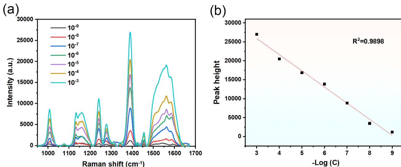
Fig. 8 (a) shows SERS spectrum of 10^{-3} – 10^{-9} M diphenyl phthalate (DHPH); (b) shows linear fitting of the negative logarithm of the AgNPs/CuNPs/Bragg-PSi substrate to the DHPH solution concentration and its Raman peak intensity at 1388 \text{ cm}^{-1} .
