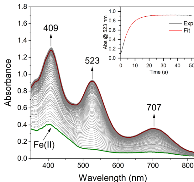
Fig. 1 Time-resolved spectral changes obtained upon mixing THF solutions of five-coordinate [\text{Fe}^{\text{II}}(\text{S}_2^{\text{Me}_2\text{N}_3(\text{Pr,Pr}))}] (1, 0.25 mM) and O 2 (3.95 mM) at -40 \text{ }^\circ\text{C} . Inset: kinetic trace ( \lambda = 523 \text{ nm} ) showing the formation of the Fe-O 2 intermediate 2. All reported concentrations are after mixing in the stopped-flow cell.
