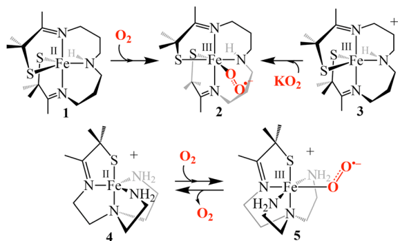
Scheme 1 Pathways for the formation of [\text{Fe}^{\text{III}}(\text{S}_2^{\text{Me}_2\text{N}_3(\text{Pr,Pr}))}(\text{O}_2)] (2) (top), and reversible dioxygen binding to [\text{Fe}^{\text{II}}(\text{S}^{\text{Me}_2\text{N}_4(\text{tren}))}]^+ (4) to form a putative superoxo intermediate [\text{Fe}^{\text{III}}(\text{S}^{\text{Me}_2\text{N}_4(\text{tren}))}(\text{O}_2)]^+ (5) (bottom).
