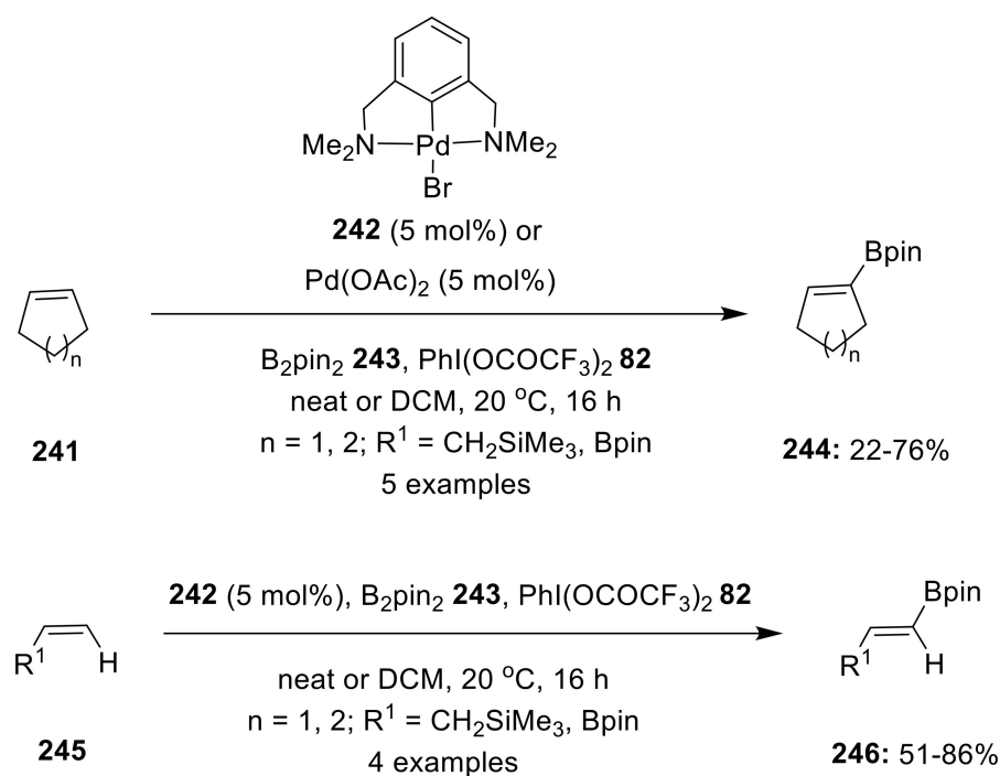
Scheme 76. Palladium-catalyzed C—H borylation of olefins 241 and 245 with B 2 pin 2 243 using PhI(OCOCF 3 ) 2 82 as an oxidant.
