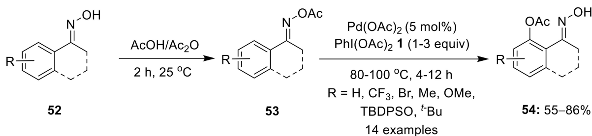
Scheme 15. Pd(II)-catalyzed O-acetyl oxime-directed C( sp^2 )—H acetoxylation of 52 to give acetoxy-lated product 54 using PhI(OAc) 2 1 .
