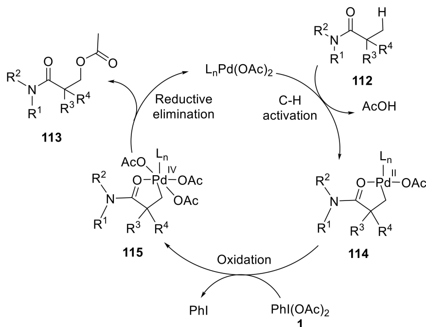
Scheme 36. Plausible reaction mechanism for acetoxylation of C(sp 2 )—H and C(sp 3 )—H bonds of tertiary amides.
