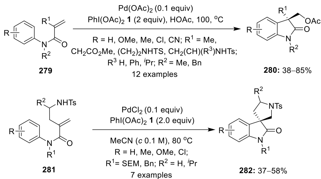
Scheme 86. Pd(II)-catalyzed synthesis of oxindoles 280 and spirooxindoles 282 from N-aryl acrylamides 279 and 281 , respectively, using \text{PhI(OAc)}_2 1 oxidant.
