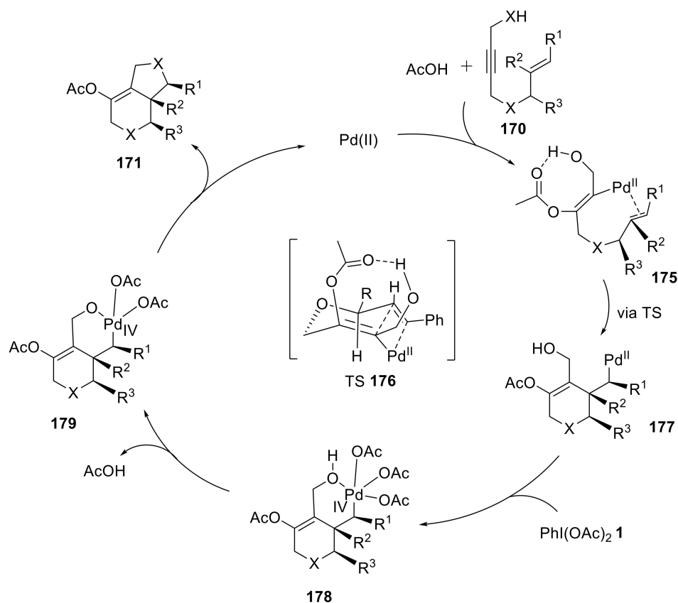
Scheme 54. The catalytic cycle for the Pd(II)-catalyzed synthesis of bicyclic heterocycles 171 from 1,6-enynes 170 using \text{PhI}(\text{OAc})_2 1 .
