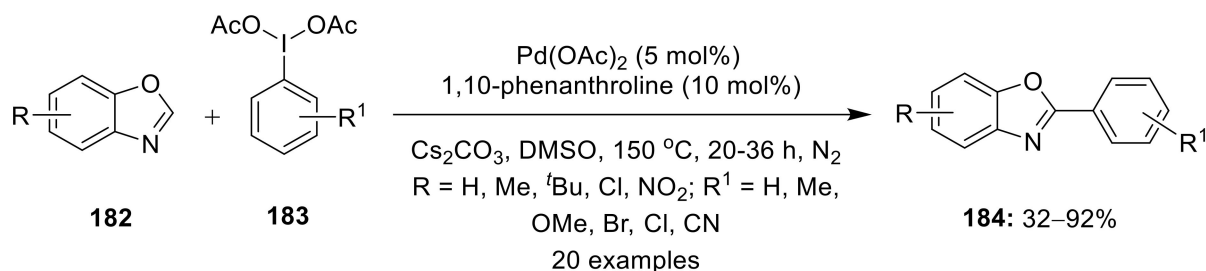
Scheme 56. Palladium-catalyzed C—H arylation of benzoxazoles derivatives 182 employing iodobenzene diacetates 183 as an arylating agent.
