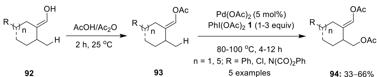
Scheme 28. Pd(II)-catalyzed O-acetyl oxime-directed \text{sp}^3 C—H acetoxylation of 92 to give acetoxy-lated products 94 using \text{PhI(OAc)}_2 1 as oxidant.
