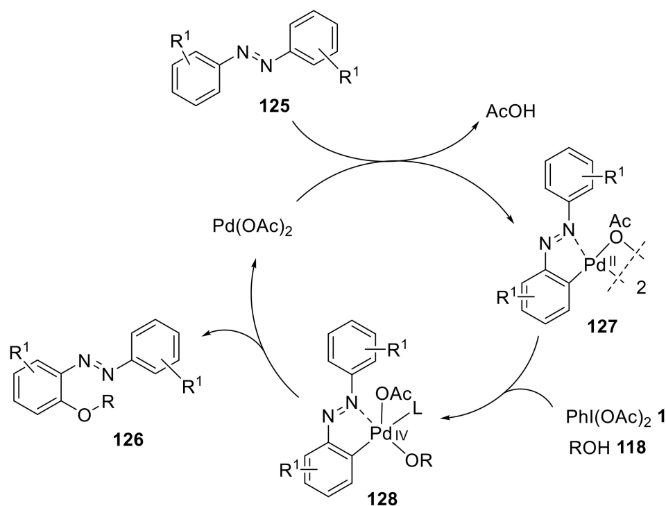
Scheme 40. The plausible catalytic cycle for the palladium-catalyzed C(sp 2 )-H-alkoxylation of azobenzene derivatives 125 using PhI(OAc) 2 1 .
