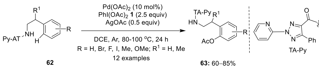
Scheme 18. Pd(II)-catalyzed C—H activation of TA-Py-directed 62 to afford acetoxyated products 63 using \text{PhI}(\text{OAc})_2 1 .
