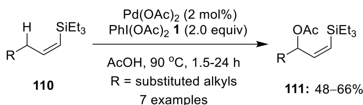
Scheme 34. Pd(II)-catalyzed allylic oxidation of cis-vinylsilanes 110 to provide products 111 employing the PhI(OAc) 2 1 oxidant.
