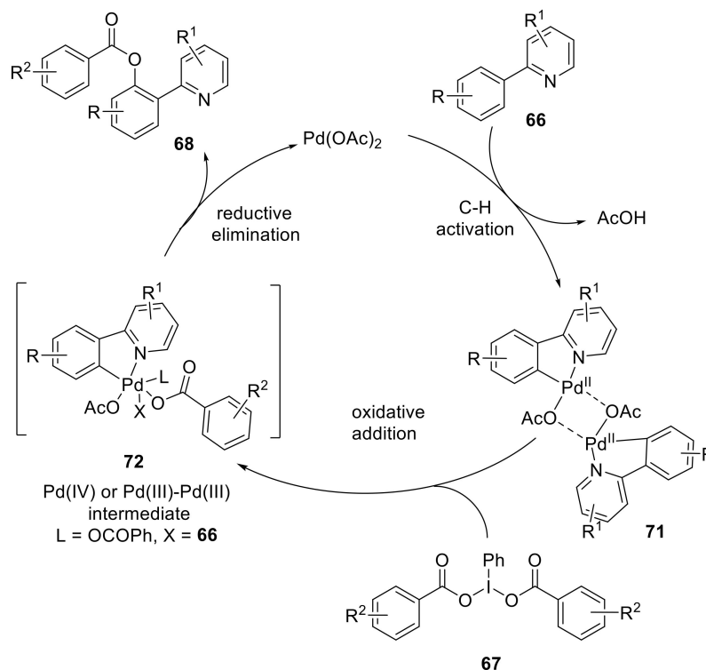
Scheme 21. Plausible catalytic cycle for the Pd(II)-catalyzed ortho-C—H benzoxylation of 66 using iodobenzene dibenzoates 67 .
