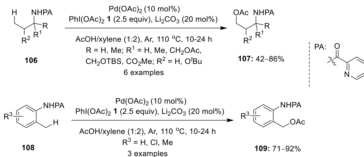
Scheme 33. Pd(II)-catalyzed \gamma -C(sp 3 )—H acetoxylation of PA-directed substrates 106 and 108 using PhI(OAc) 2 1 as the oxidant.
