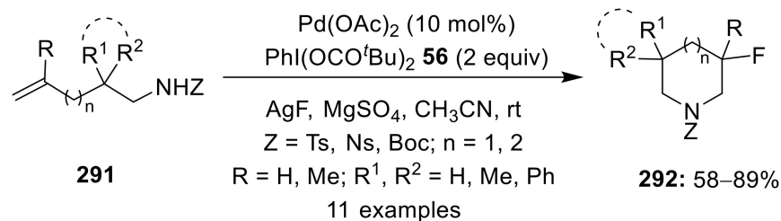
Scheme 89. Pd(II)-catalyzed intramolecular aminofluorination of olefins 291 to afford cyclic amines 292 using oxidant \text{PhI}(\text{OCO}^t\text{Bu})_2 56 .
