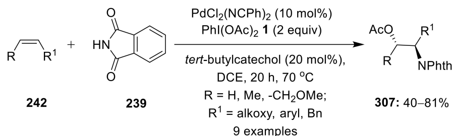
Scheme 95. Pd(II)-catalyzed intermolecular aminoacetoxylation of alkenes 242 using \text{PhI}(\text{OAc})_2 1 .
