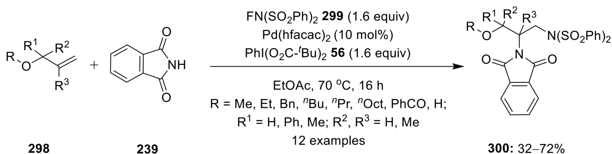
Scheme 92. Pd(II)-catalyzed intermolecular 1,2-diamination of allylic ethers 298 with phthalimide 239 and N-fluoro-bis(phenylsulfonyl)imide 299 as nitrogen sources.
