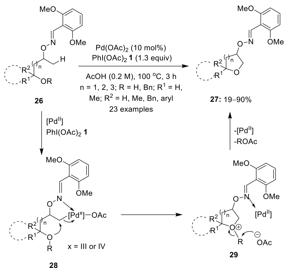
Scheme 6. Pd(II)-catalyzed preparation of cyclic ethers 27 from oxime-masked alcohols 26 using \text{PhI(OAc)}_2 1 oxidant.
