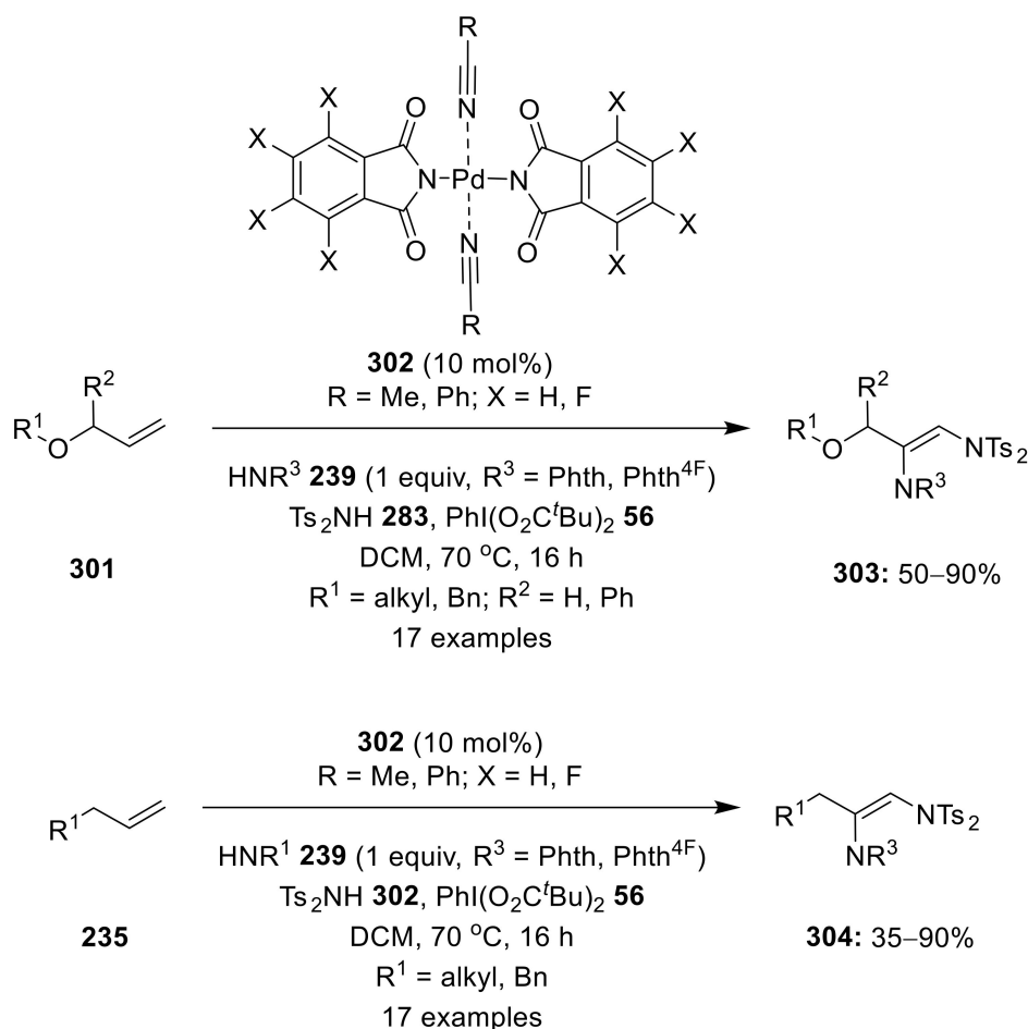
Scheme 93. Pd(II)-catalyzed diamination of allyl ethers 301 and alkenes 235 using \text{PhI(O}_2\text{CtBu)}_2 56 as an oxidant.
