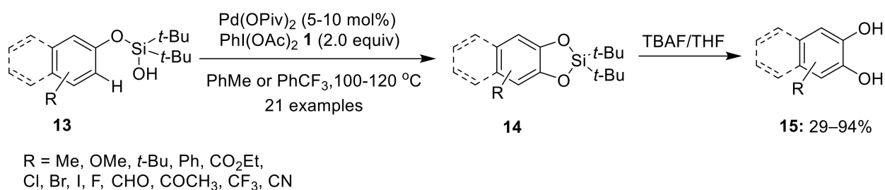
Scheme 3. Pd(II)-catalyzed synthesis of substituted catechols 15 from silanols 13 using PhI(OAc) 2 1 as oxidant.
