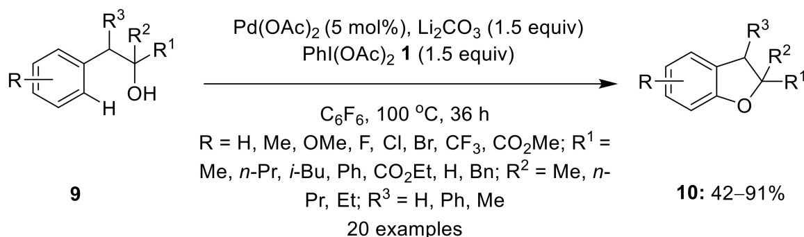
Scheme 1. Pd-catalyzed synthesis of dihydrobenzofurans 10 via hydroxyl-group directed C—H activation/C—O cyclization reaction of 9 using \text{PhI(OAc)}_2 1 as terminal oxidant.
