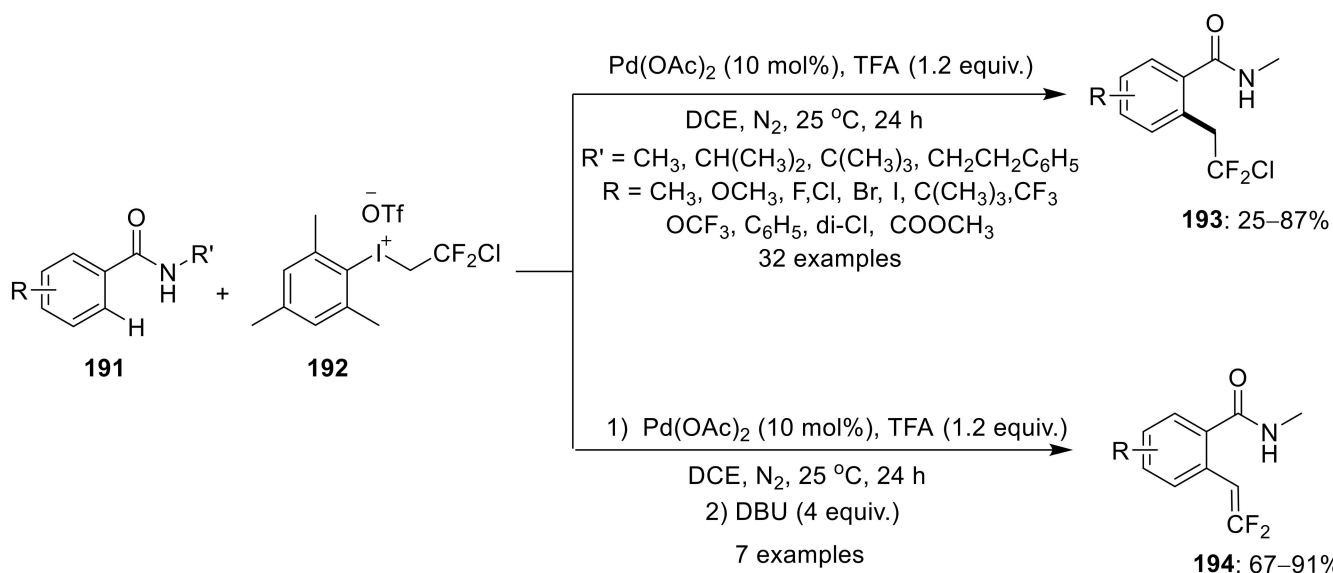
Scheme 59. Pd-catalyzed synthesis of difluoroethyl 193 and difluorovinyl 194 compounds from substituted aromatic amides 191 using chlorodifluoroethyl idonium salt (CDFI) 192 .
