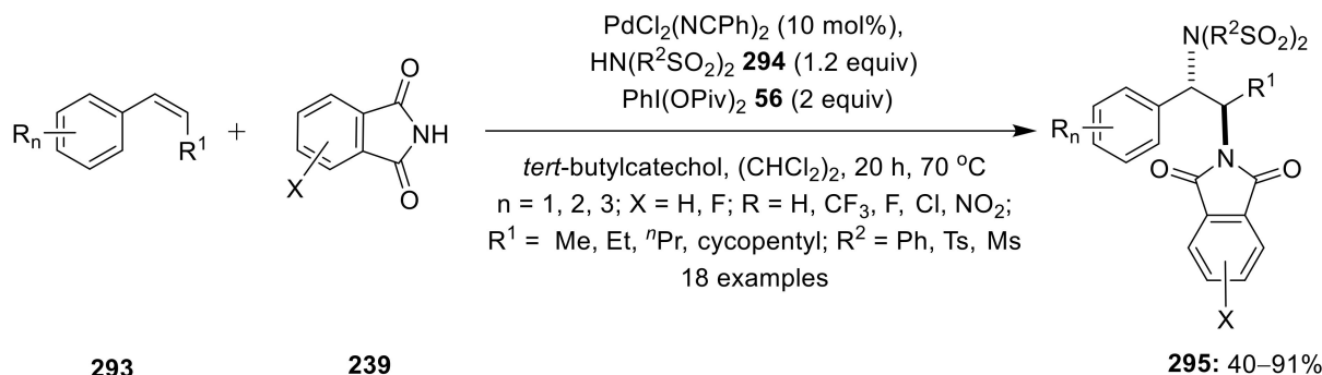
Scheme 90. Pd(II)-catalyzed intermolecular 1,2-diamination of internal alkenes 293 with phthalimide 239 and bissulfonimides 294 as a nitrogen source to desired products 295 .
