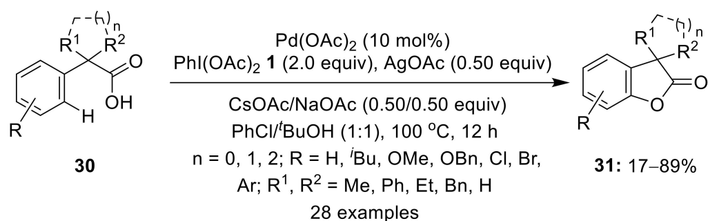
Scheme 7. Pd(II)-catalyzed direct lactonization of acids 30 to synthesize benzofuranones 31 using \text{PhI(OAc)}_2 1 as an oxidant.
