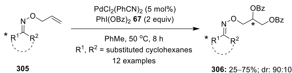
Scheme 94. Pd(II)-catalyzed oxime-directed asymmetric 1,2-dioxygenation chiral oxime allyl ether 305 with \text{PhI}(\text{OBz})_2 67 .
