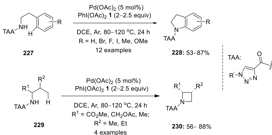
Scheme 72. Pd(II)-catalyzed C—H activation of TAA-directed substrates 227 and 229 to cyclic products 228 and 230 , respectively, using \text{PhI(OAc)}_2 1 as an oxidant.
