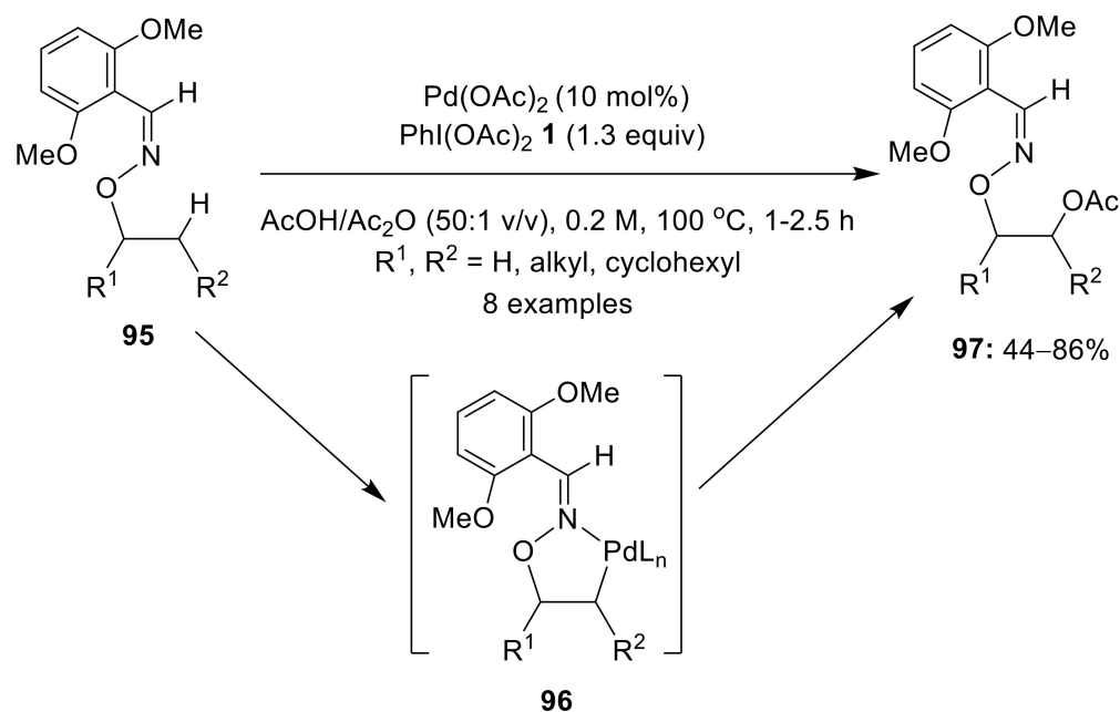
Scheme 29. Pd(II)-catalyzed site-selective \text{C}(\text{sp}^3) —H acetoxylation of 95 to provide protected 1,2-diols 97 using oxidant \text{PhI(OAc)}_2 1 .
