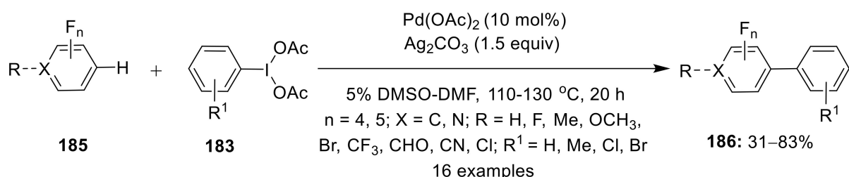
Scheme 57. \text{Pd(OAc)}_2 -catalyzed C—H arylation of polyfluoroarenes 185 using aryl iodine(III) diacetates 183 as aryl source to afford coupled products 186 .
