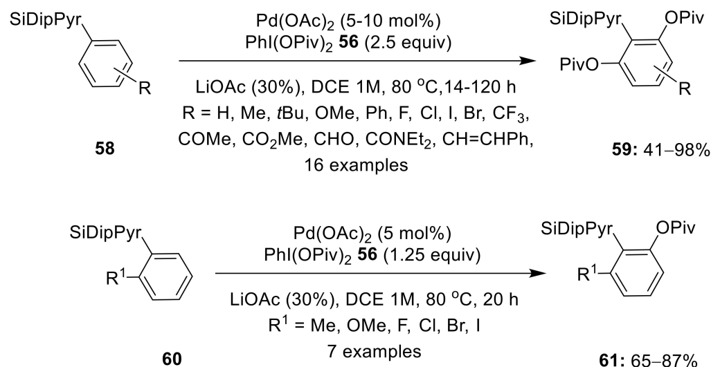
Scheme 17. Pd(II)-catalyzed 2-pyrimidyl-diisopropylsilyl-directed C—H oxygenation of arenes 58 and 60 to products 59 and 61 , respectively, using \text{PhI}(\text{OPiv})_2 56 as an oxidant.
