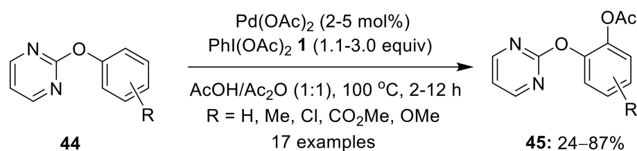
Scheme 12. \text{Pd}(\text{II}) -catalyzed pyrimidine-directed ortho-acetoxylation of phenol derivatives 44 using \text{PhI}(\text{OAc})_2 1 as an oxidant to form acetoxyated products 45 .
