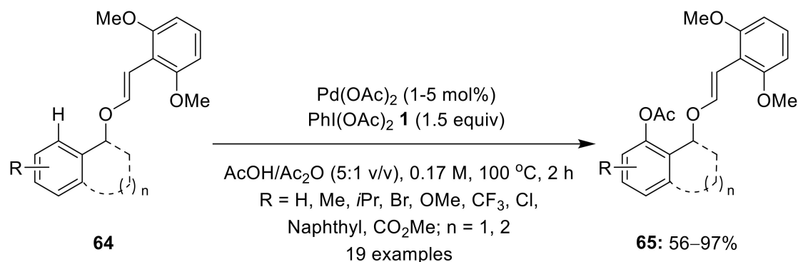
Scheme 19. Pd(II)-catalyzed dimethoxybenzaloxime-directed ortho-acetoxylation of arenes 64 to produce acetoxyated products 65 using \text{PhI}(\text{OAc})_2 1 as an oxidant.
