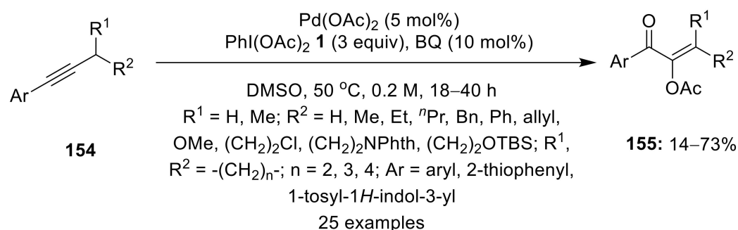
Scheme 48. Pd(II)-catalyzed acetoxylation of alkynes 154 using \text{PhI(OAc)}_2 1 as an oxidant to prepare \alpha -acetoxy enones 155 .
