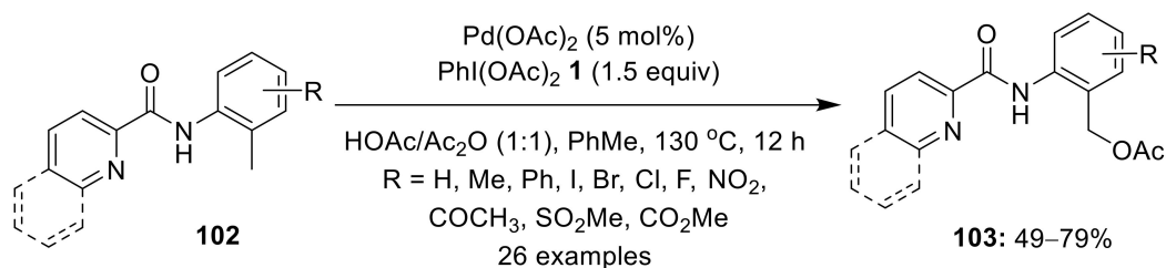
Scheme 31. Pd(II)-catalyzed acetoxylation of benzylic C—H bond of substrates 102 to afford acetoxy-lated products 103 using PhI(OAc) 2 1 as the oxidant and acetate source.
