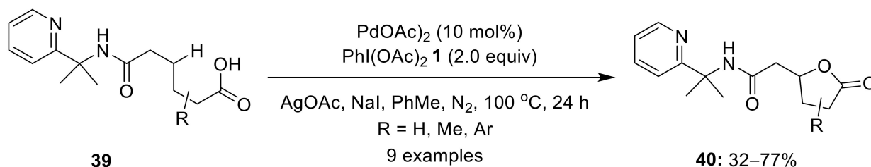
Scheme 10. Pd(II)-catalyzed synthesis of \gamma -lactones 40 through PIP auxiliary-directed intramolecular lactonization of aliphatic acids 39 using PhI(OAc) 2 1 as oxidant.
