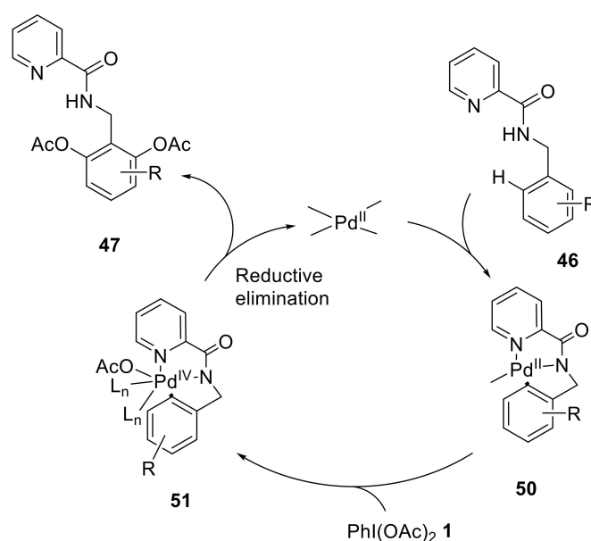
Scheme 14. Plausible catalytic cycle for the Pd(II)-catalyzed ortho-acetoxylation of arenes 46 to 47 using \text{PhI}(\text{OAc})_2 1 as an oxidant.
