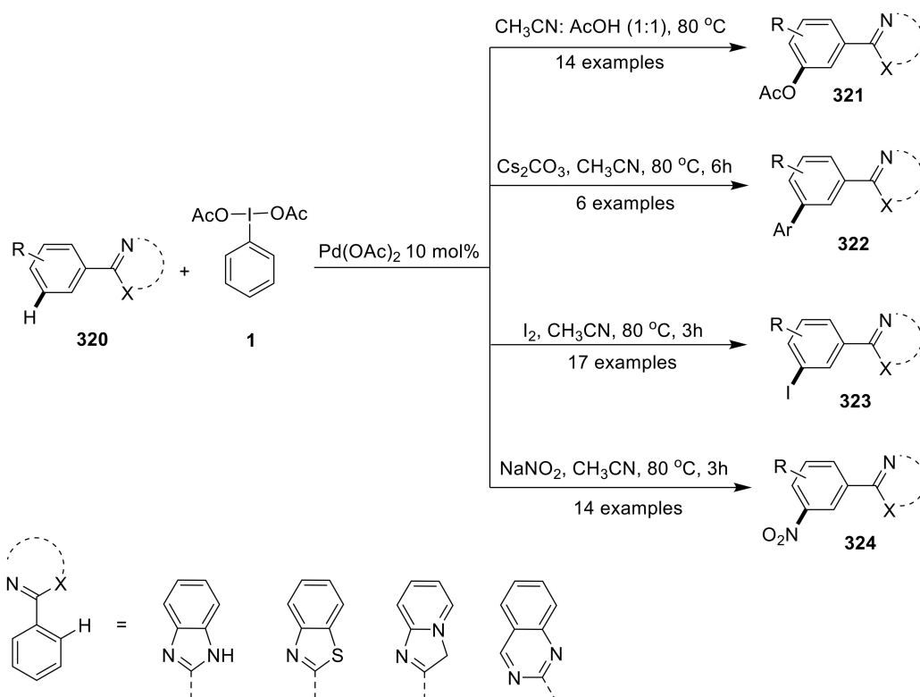
Scheme 99. Pd-catalyzed C(sp 2 )—H functionalization of benzothiazole/benzoxazole/benzimidazole 320 using PIDA 1 as an oxidant.
