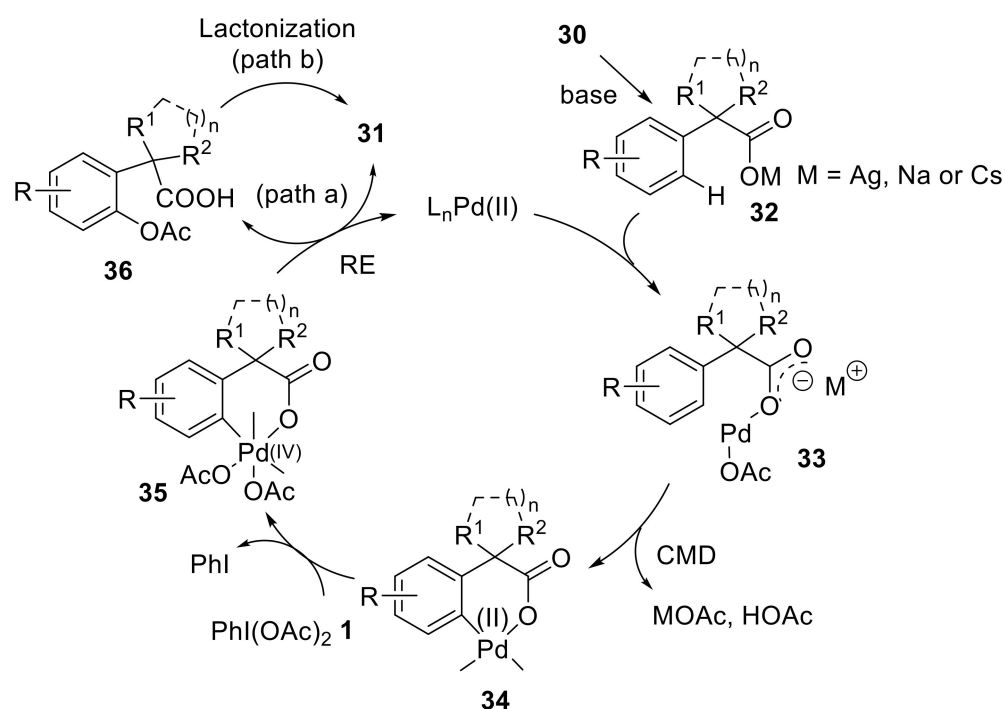
Scheme 8. The catalytic cycle for the intramolecular lactonization of acids 30 to synthesize benzofurones 31 using PhI(OAc) 2 1 as an oxidant.
