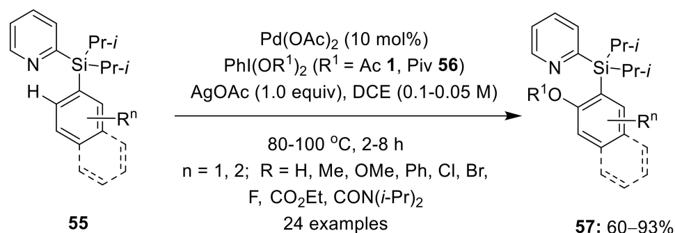
Scheme 16. Pd(II)-catalyzed pyridyldiisopropylsilyl-directed C—H acyloxylation of arylsilanes 55 using PhI(OAc) 2 1 or PhI(OPiv) 2 56 as an oxidant and acyloxyl group source.
