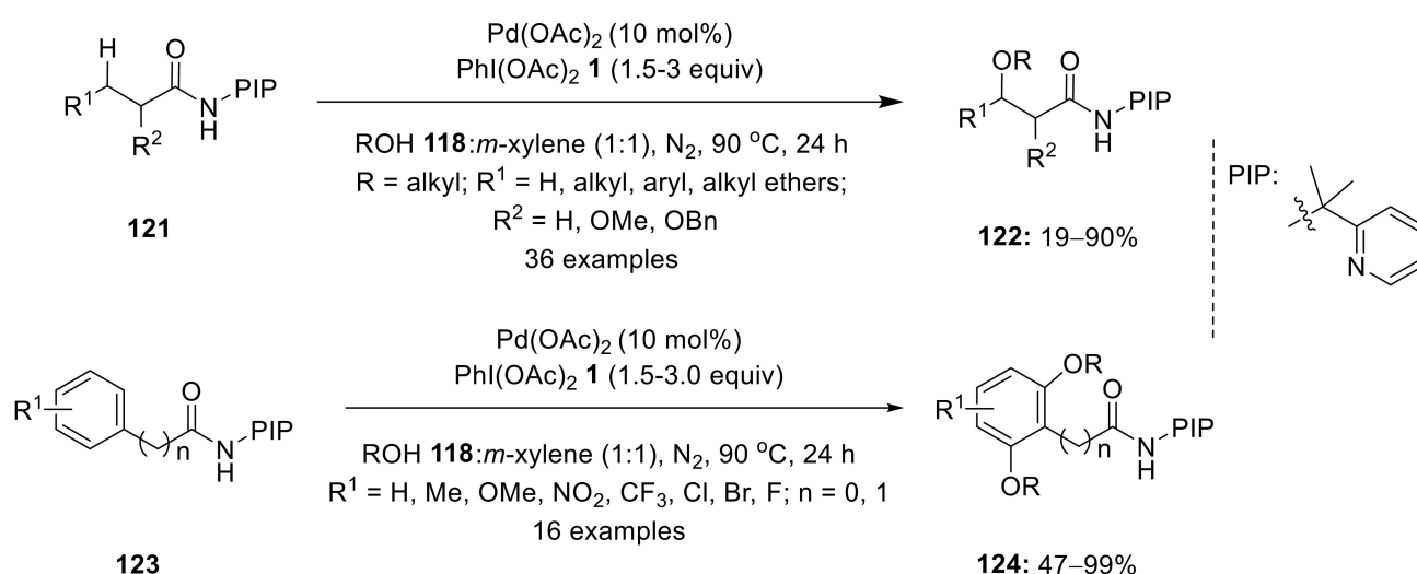
Scheme 38. Pd(II)-catalyzed \text{PhI}(\text{OAc})_2 -mediated C—H alkoxylation of unactivated \text{C}(\text{sp}^3) —H and \text{C}(\text{sp}^2) —H bond of substrates 121 and 123 to alkoxylation products 122 and 124 , respectively.
