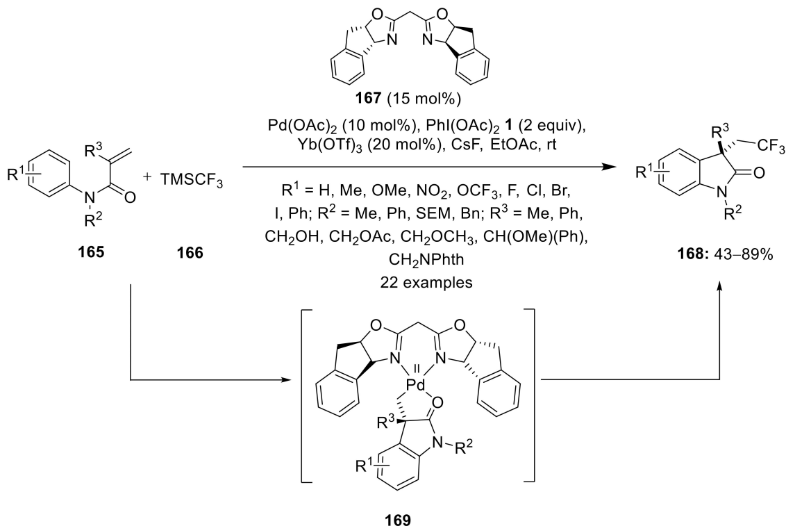
Scheme 52. Pd(II)-catalyzed intramolecular trifluoromethylation activated alkenes 165 with TMSCF 3 166 as trifluoromethyl source to deliver CF 3 -substituted oxindoles 168 .
