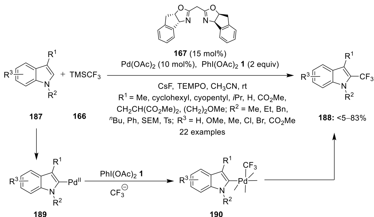
Scheme 58. Pd-catalyzed C—H trifluoromethylation of 187 to yield trifluoromethylated products 188 using TMSCF 3 166 as CF 3 source and PhI(OAc) 2 1 as an oxidant.
