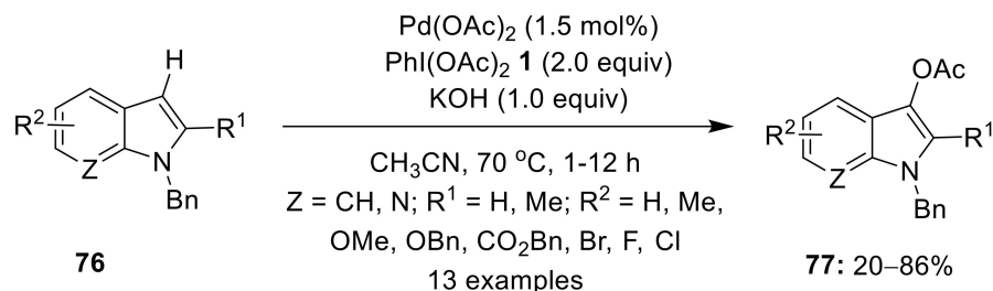
Scheme 23. Pd(II)-catalyzed C3-acetoxylation of substituted indoles 76 to afford C3-acetoxyated indoles 77 using PhI(OAc) 2 1 .
