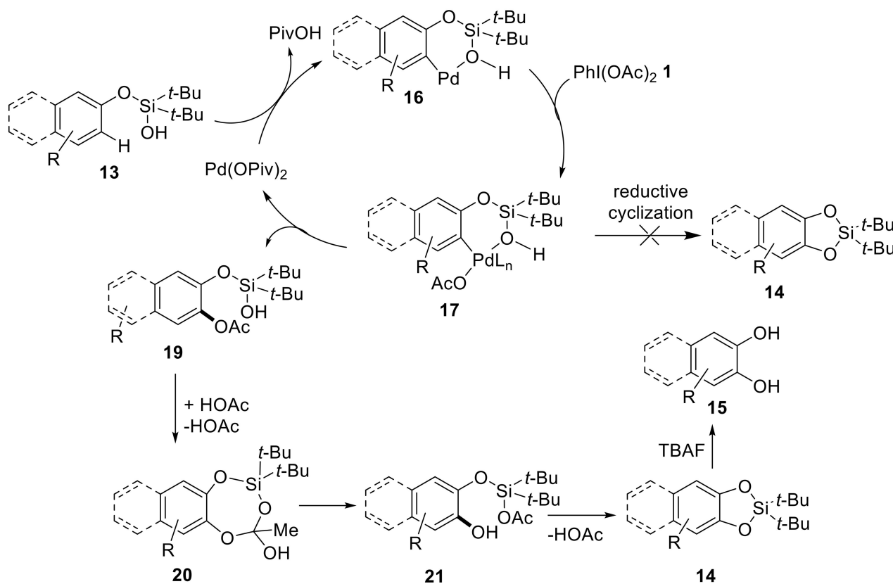
Scheme 4. Plausible catalytic cycle for the synthesis of substituted catechols 15 via C—H oxygenation of silanols 13 using oxidant PhI(OAc) 2 1 .
