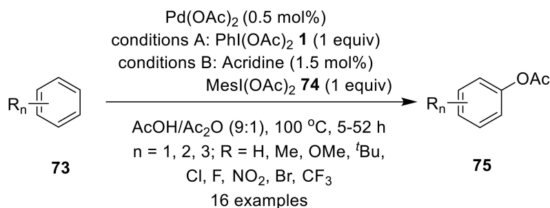
Scheme 22. Pd-catalyzed site-selective C—H acetoxylation of multi-substituted arenes 73 using oxidant PhI(OAc) 2 1 or MesI(OAc) 2 74 .
