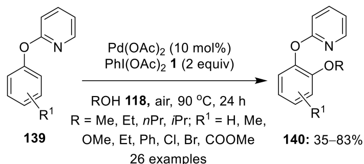
Scheme 43. Pd(II)-catalyzed ortho-alkoxylation of 2-aryloxy pyridines 139 using alcohols 118 as source of an alkoxy group and PhI(OAc) 2 1 as an oxidant.
