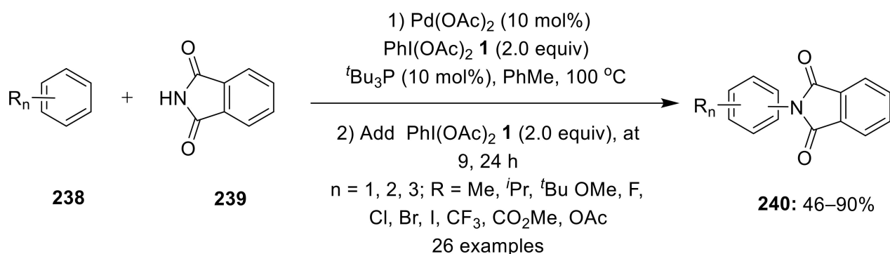
Scheme 75. Pd(II)-catalyzed intermolecular C—H amination of multi-substituted arenes 238 with phthalimide 239 using \text{PhI(OAc)}_2 1 as an oxidant.
