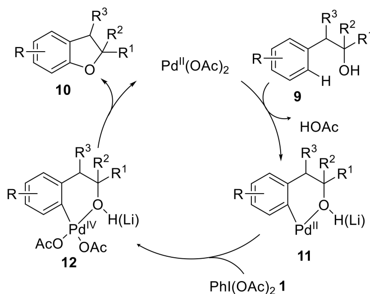
Scheme 2. Plausible catalytic cycle for the Pd(II)-catalyzed synthesis of dihydrobenzofurans 10 using \text{PhI(OAc)}_2 1 as a terminal oxidant.
