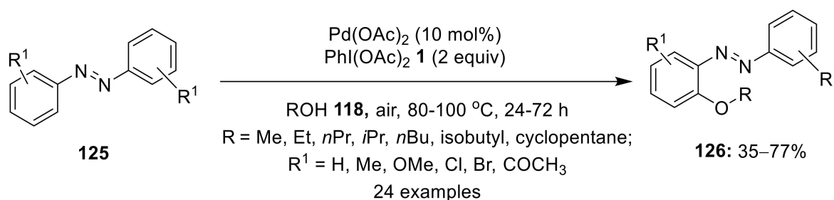
Scheme 39. Palladium-catalyzed \text{PhI}(\text{OAc})_2 -mediated \text{C}(\text{sp}^2) —H alkoxylation of azobenzene derivatives 125 to afford ortho-alkoxylation products 126 .
