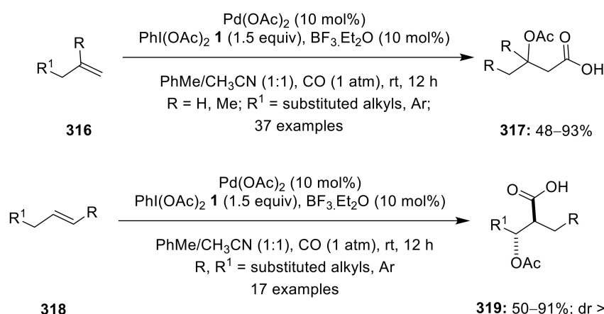
Scheme 98. Pd(II)-catalyzed oxycarbonylation of alkenes 316 and 318 using PhI(OAc) 2 1 as oxidant.
