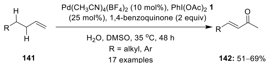
Scheme 44. Pd(II)/Iodine(III)-catalyzed Wacker oxidation–dehydrogenation of olefins 141 to afford \alpha, \beta -unsaturated ketones 142 using \text{PhI}(\text{OAc})_2 1 as a cocatalyst.
