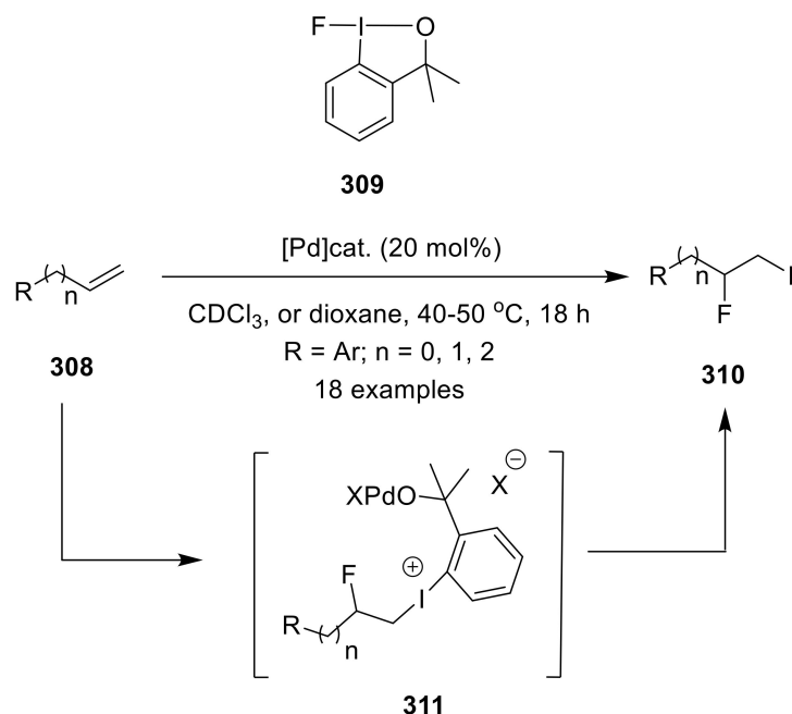
Scheme 96. Pd(II)-catalyzed intermolecular iodofluorination of alkenes 308 using PhI(OAc) 2 1 .
