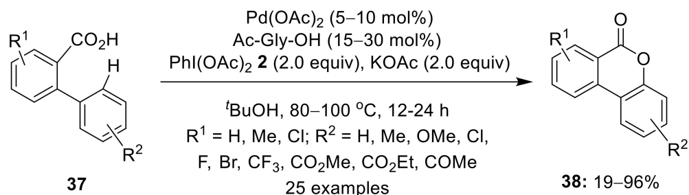
Scheme 9. Pd(II)-catalyzed C—H activation/C—H cyclization of biaryl carboxylic acids 37 to afford biaryl lactones 38 using PhI(OAc) 2 1 .
