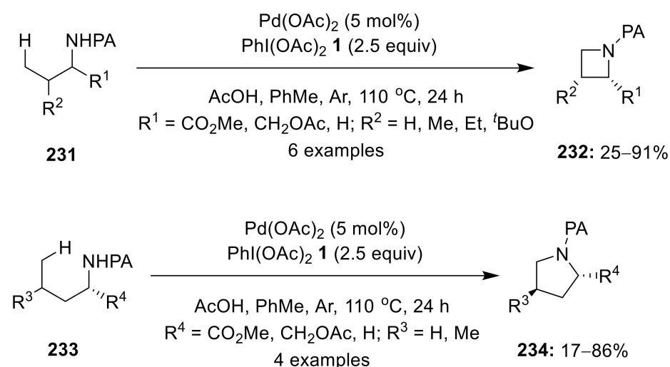
Scheme 73. Pd(II)-catalyzed intramolecular C—H amination of PA-directed amine substrates 231 and 233 , azetidines 232 , and pyrrolidines 234 , respectively, using \text{PhI(OAc)}_2 1 as an oxidant.
