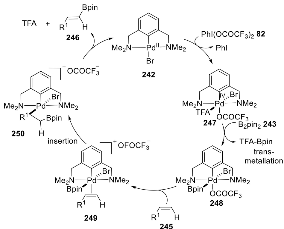
Scheme 77. Catalytic cycle for the palladium pincer complex-catalyzed C—H borylation of olefins 245 using PhI(OCOCF 3 ) 2 82 as an oxidant.
