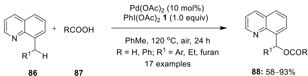
Scheme 26. Pd(II)-catalyzed chelation-assisted \text{C}(\text{sp}^3)\text{-H} acyloxylation of 86 with carboxylic acids 87 using \text{PhI}(\text{OAc})_2 1 as an efficient oxidant.
