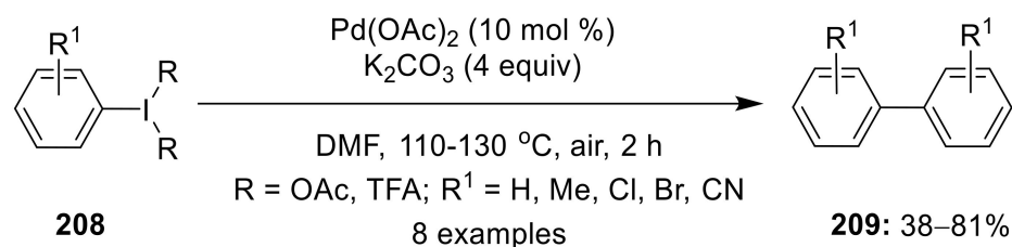
Scheme 65. Pd(II)-catalyzed homocoupling of aryliodine(III) diacetate 208 to furnish desired biaryls 209 .
