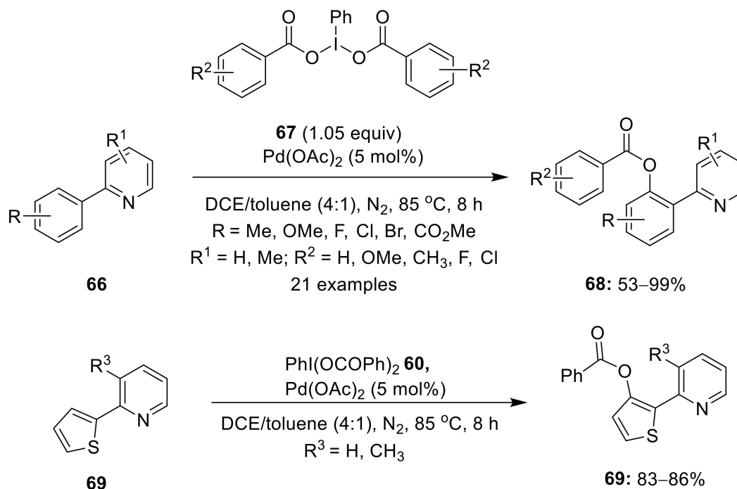
Scheme 20. Pd(II)-catalyzed ortho C—H benzylation of 66 and 69 using substituted iodobenzene dibenzoates derivatives 67 as oxidant and source of benzoyl group.
