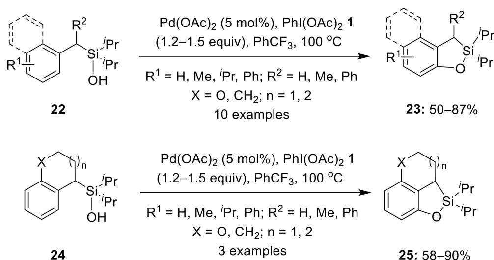
Scheme 5. Pd(II)-catalyzed C—H oxygenation of benzylsilanol 22 and 24 to oxasilacycles 23 and 25 , respectively, using \text{PhI}(\text{OAc})_2 1 as oxidant.
