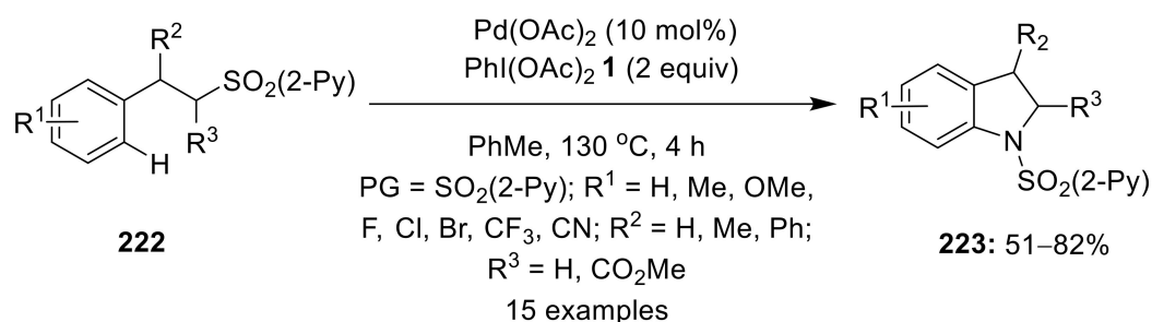
Scheme 70. Pd(II)-catalyzed synthesis of indolines 223 via C—H activation/C—H cyclization of phenethylamine derivatives 222 using \text{PhI(OAc)}_2 1 as an oxidant.
