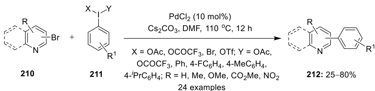
Scheme 66. Pd(II)-catalyzed arylation of N-heteroaromatic bromides 210 to access arylated heteroaromatic compounds 212 using hypervalent iodine(III) reagents 211 .
