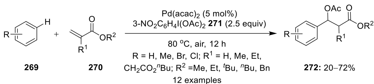
Scheme 83. Pd(II)-catalyzed 1,1-difunctionalization of activated olefins 270 with substituted arenes 269 using oxidant 3\text{-NO}_2\text{C}_6\text{H}_4\text{I(OAc)}_2 271 .
