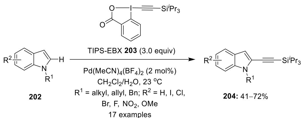
Scheme 63. Pd(II)-catalyzed regioselective C2-alkynylation of N -alkylated indoles 202 using TIPS-EBX 203 as an alkynyating reagent.
