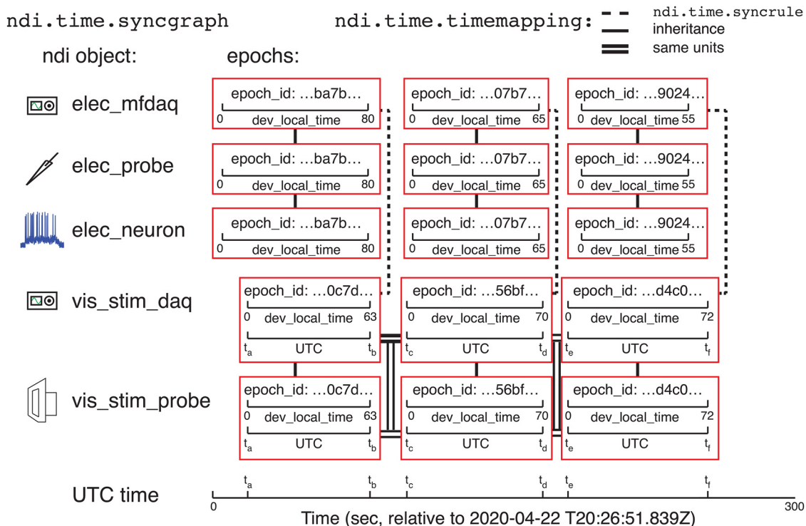
Figure 7. Epochs and ndi.time.syncgraph . Illustration of an example experiment similar to that in Figure 6, except that the vis_stim_daq DAQ system also keeps UTC time in addition to its own local clock. Here, time can be converted among any epoch because there is a mapping between the epochs of vis_stim_daq and UTC, and there are ndi.time.timemapping mappings between the DAQ system. The time in any epoch can be computed according to the clock of any other epoch, by solving the transformations in the syncgraph. The mappings shown are ndi.time.timemapping objects built by (1) an ndi.time.syncrule ; (2) inheritance (e.g., a probe inherits the epoch information of the DAQ system that acquired it); and (3) same units (UTC is a global time system).
