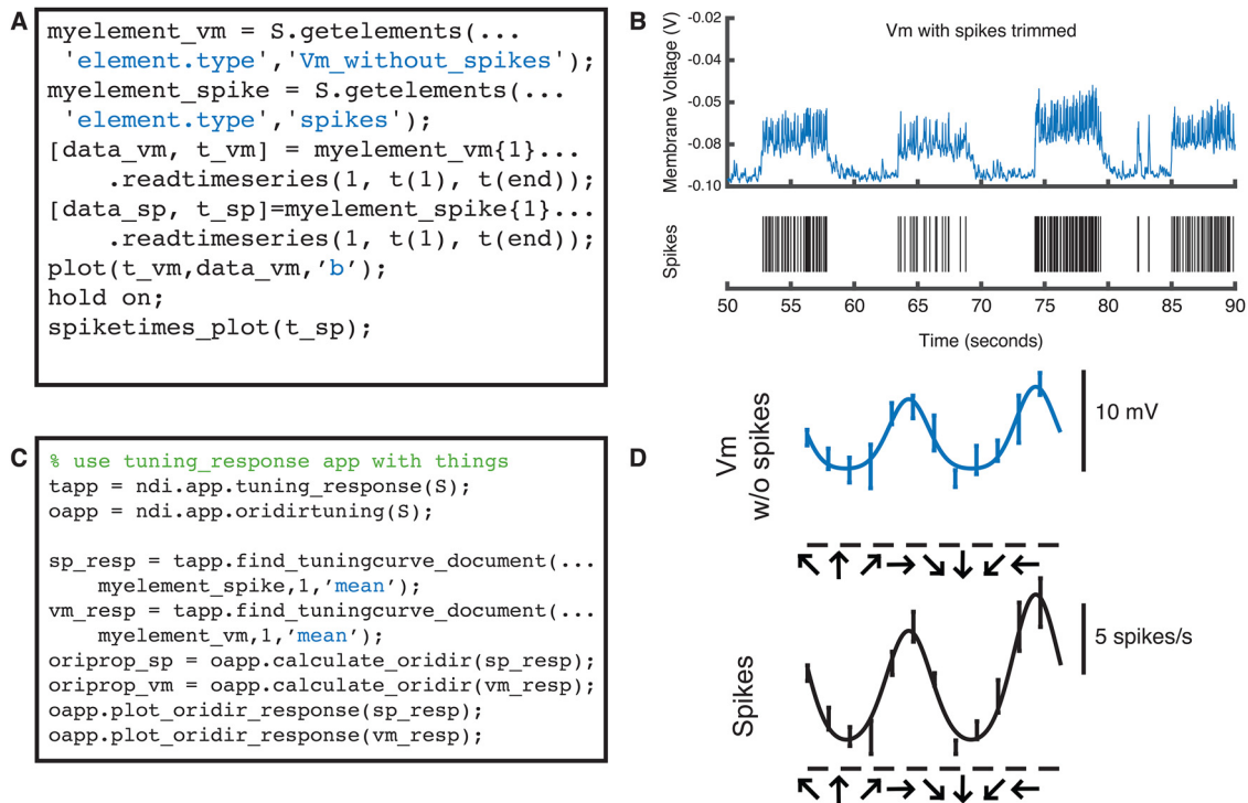
Figure 5. ndi.element objects allow different types of data to go through identical analysis pipelines. Code that reads (A) and plots (B) time series data from 2 ndi.element objects derived from a single sharp electrode probe: voltage membrane data where spikes have been “chopped” out with a median filter (top) and thresholded spike data (bottom). C, The objects can be sent through analysis applications identically and the same type of summary data generated and plotted. D, Orientation and direction tuning curves for the subthreshold membrane voltage and spiking activity of the same cell. Note that filtered data, modeled data, or artificial test data can be sent through the same analysis pipelines with ndi.element .
