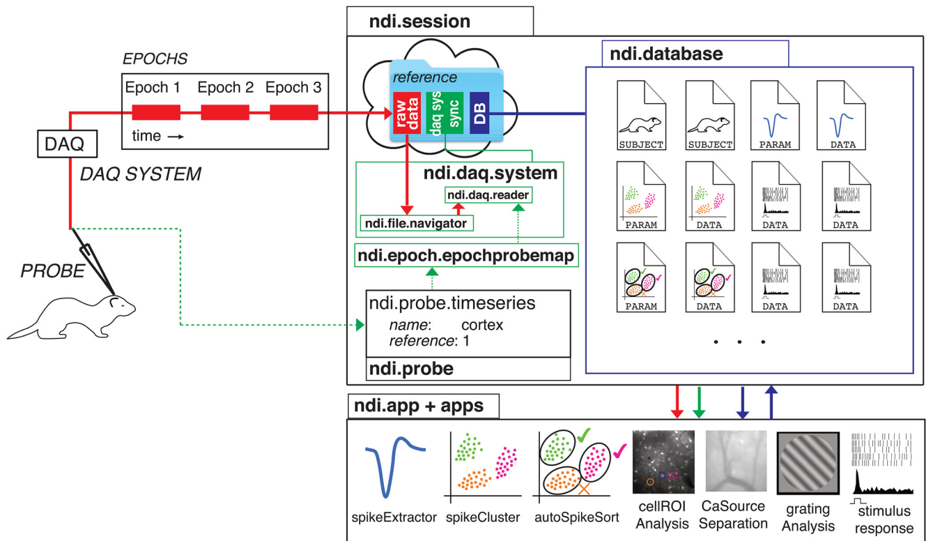
Figure 2. An overview of the NDI. Top left, The physical experiment from Figure 1. A probe (electrode) is used to sample data from the visual cortex of a subject ferret. A DAQ system digitally logs the measurements. Three epochs of data have been recorded by the DAQ system. Top right, An experiment session is contained in a software object that has a link to the raw data (red), an internal set of NDI objects that have information about DAQ systems and synchronization methods (green), and link to a database (dark blue). Upon creation, each ndi.daq.system object is provided with an ndi.file.navigator object, which is a parameterized set of instructions for locating the raw files or links that contain the data for a given epoch. Therefore, the same ndi.daq.system can manage data that is organized into epochs on disk according to different schemas. Metadata associated with each epoch, in a type called ndi.epoch.epochprobemap , specifies the probes that are present in each recorded epoch and indicates the probe's name, a unique reference, and the channel mapping between the ndi.daq.system and the probe. This data can be added manually by the user or analyst, or can be read from the epoch data files if the ndi.daq.system 's data format or a LIMS encodes this information. The database stores documents, which are platform-independent representations of analyses, analyses of analyses, and NDI internal objects. Bottom right, Applications can use NDI to read raw data and read the results of previous analyses from the database and write the results of new analyses back to the database as documents. The database and documents therefore support the construction of pipelines that may be linear or integrated. Applications are free to focus on single analysis problems instead of the raw data format or organization of their input.
