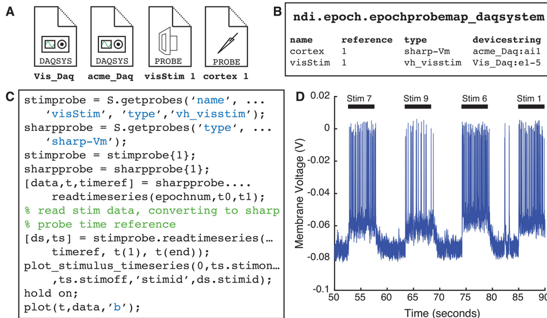
Figure 4. Probes. A , When probes are defined by providing (B) a mapping between the channels of the probe and the channels of the DAQ system, the data can be read through direct calls, and NDI manages the necessary calls to the DAQ systems. C , Code snippet that loads probe objects for a visual stimulus system and a sharp electrode, and reads time series data from the sharp electrode probe. The code returns a time reference for the sharp probe’s epoch, and that reference is used to request a time series with the corresponding time intervals from the visual stimulus system (although the systems likely do not have the same clocks). D , The raw data and stimulus information are plotted together.
