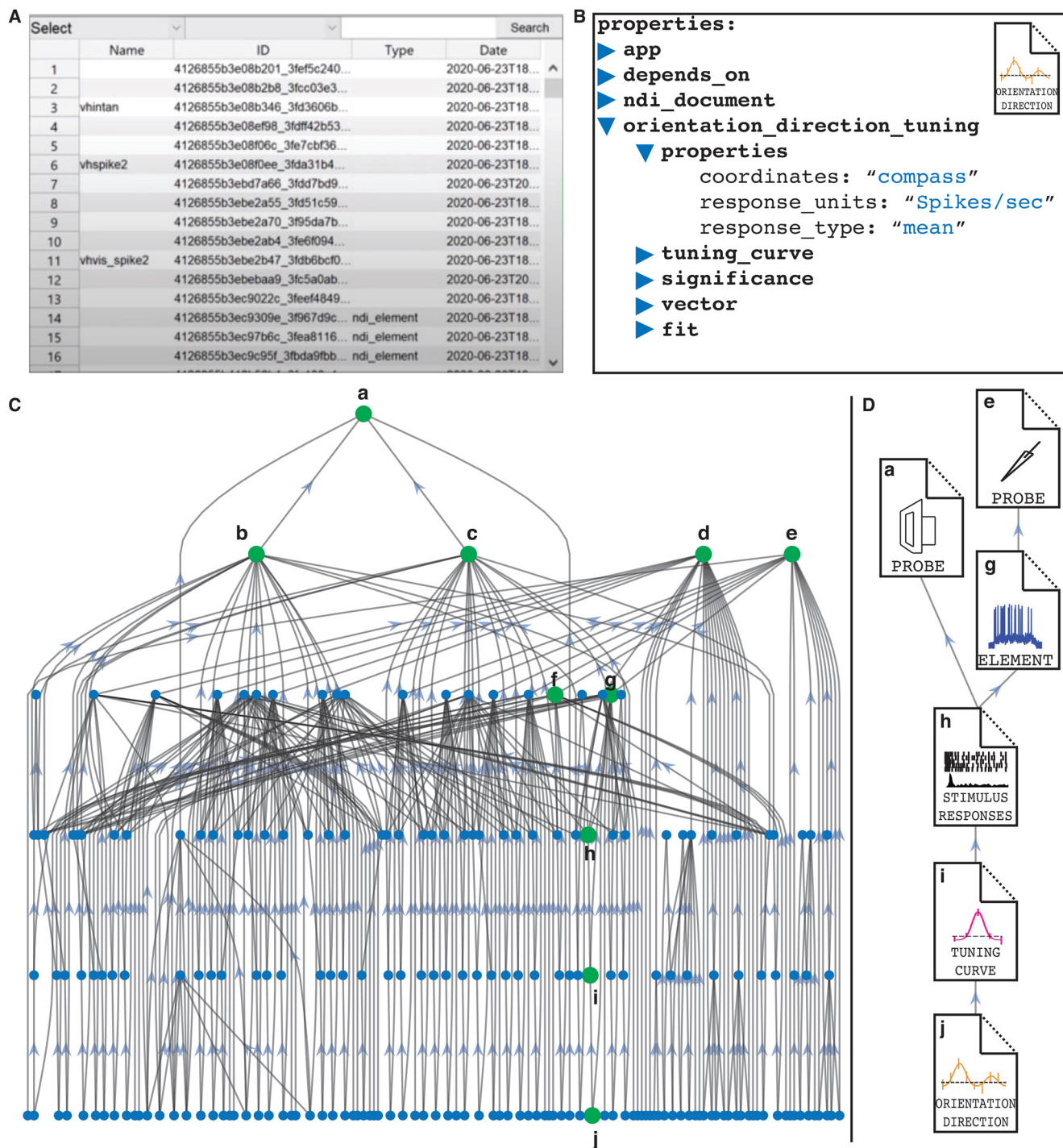
Figure 11. Graph structure of the database documents of an example experimental session, Roy et al. (2020) in NDI. A , linear list of documents with IDs. B , Property view of a document that stores information about orientation and direction tuning. C , Full graph of documents. Documents are denoted by nodes (blue or green circles), and arrows point from dependent documents to the documents that they depend on. In this graph, a is a visual stimulus monitor probe, and b , c are stimulus presentation documents that describe the presentation of sinusoidal gratings in different directions. d , e are sharp electrode probes corresponding to two recordings of different impaled cells. f , g are documents describing the ndi.element objects of probe e where spikes are removed ( f ) and where spike times are extracted ( g ). h is a document containing the stimulus responses of the spikes in g to the stimulus presentation in c . In i , these stimulus responses have been collated into a tuning curve. Finally, these responses have been examined to extract orientation and direction index values and to perform a double Gaussian fit, which are all stored in document j . D , Zoomed in view of the document pipeline a-j .
