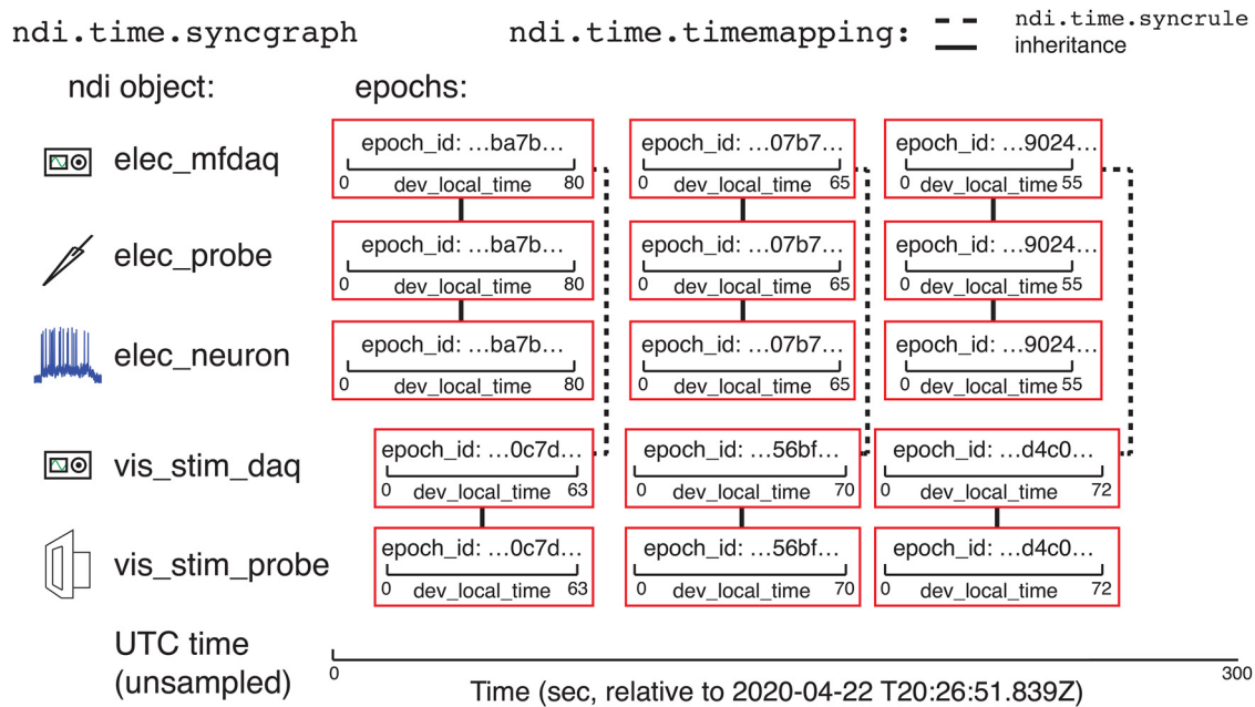
Figure 6. Epochs and ndi.time.syncgraph . Illustration of an example experiment with two ndi.daq.system objects ( elec_mfdaq and vis_stim_daq ) that are each connected to a probe ( elec_probe and vis_stim_probe , respectively). The DAQ systems have their own clocks that are not linked to any global time system. Three epochs have been recorded by each DAQ system. The electrode probe has been analyzed and an ndi.element object (a neuron, elec_neuron ) has been created from it. The clock and time of each of the epochs for the neuron is inherited from its underlying probe, which is in turn inherited from the underlying DAQ system. The two DAQ systems each record the same set of digital triggers, and ndi.time.syncgraph has used its list of ndi.time.syncrule objects to compute a mapping ( ndi.time.timemapping ) between epochs of those DAQ systems. Time can be converted between epochs that are recorded simultaneously on the two DAQ systems, but we do not know how the other epochs are related to each other, or how any epoch is related to a global time system like UTC, shown below.
