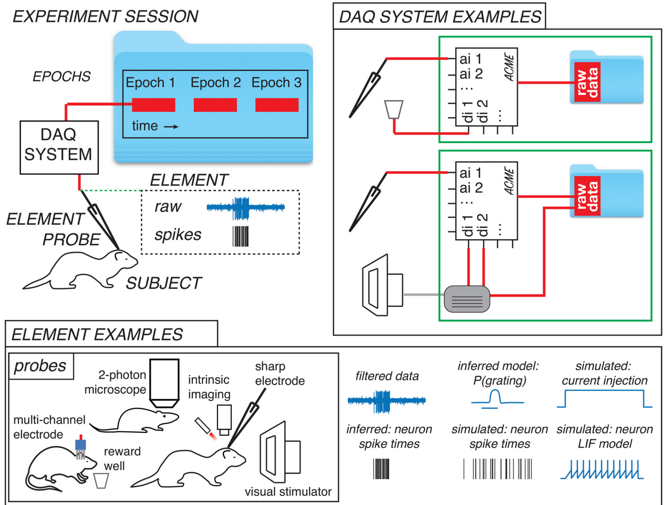
Figure 1. A vocabulary for neuroscience experiments that forms the basis of the NDI. Top left, An example experiment. A probe is any instrument that can make a measurement from or provide stimulation to a subject. In this case, an electrode with an amplifier is monitoring signals in cerebral cortex of a ferret and the electrode is a probe and the ferret is a subject. A DAQ system is an instrument that digitally logs the measurements or stimulus history of a probe. In this case, a DAQ is logging the voltage values produced by the electrode’s amplifier and storing the results in a file on a computer. An epoch is an interval of time during which a DAQ system is switched on and then off to make a recording. In this case, three epochs have been sampled. The experiment has additional experiment elements. One of these elements is a filtered version of the electrode data. A second element is a neuron, whose existence and spike times have been inferred by a spike analysis application and recorded in the experiment. Bottom, In NDI, a wide variety of experiment items are called elements, of which probes are a subset. Examples of probes include multichannel extracellular electrodes, reward wells, two-photon microscopes, intrinsic signal imaging systems, intracellular or extracellular single electrodes, and visual stimulus monitors. Other elements include items that are directly linked to probes, such as filtered versions of signals, or inferred objects like neurons whose activity are inferred from extracellular recordings or images. Still other elements have no physical derivation, such as artificial data or purely simulated data; nevertheless, we want to be able to treat these items identically in analysis pipelines. Finally, elements might be the result of complex modeling that depends on many other experiment elements, such as an inferred phenomenological model of the amount of information that an animal has about whether a stimulus is a grating. Top right, DAQ systems digitally record probe measurements or histories of stimulator activity. In NDI, DAQ systems are logical entities, which could correspond physically to a single DAQ device made by a particular company (top), or a collection of home-brewed devices that operate together to have the behavior of a single DAQ device (bottom). In the bottom example, information from an electrode probe and digital triggers from a visual stimulation probe are acquired on a single DAQ device, but digital information from both systems (in separate files) is needed to fully describe the activity in each epoch.
