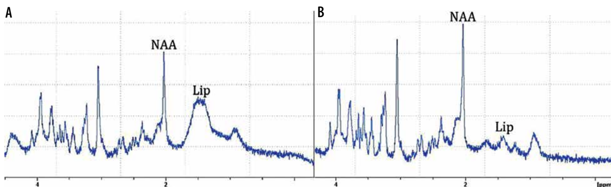
Figure 5. ^1\text{HMRS} spectrum from rat hippocampus. A) spectrum with big signal from lipids, B) spectrum with small signal from lipids. PRESS sequence: TE 16 ms, TR 2500 ms, 32 averages, VOI size 2 \times 2 \times 5.5 \text{ mm}^3 . Unwanted signals from lipids can significantly disturb spectra quality. Spectra fitting using Top Spin software, 7T Bruker, animal system
