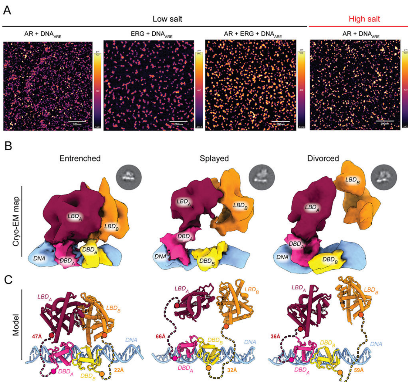
Figure 1. DNA-bound AR exhibits conformational plasticity about its dimer interfaces. (A) Representative AFM images of recombinant AR bound to DNA in the presence or absence of ERG. Scale bar at 200 nanometers. (B, C) Architecture of three distinct DNA-bound states displaying a spectrum of buried to exposed intermolecular surfaces including the Entrenched, Splayed, and Divorced conformations. (B) Cryo-EM electron density with AR domains and DNA segmented and labeled. Representative 2D classes shown above respective model. (C) Coordinate view derived from X-ray structures of LBD monomers (He et al., 2004) (PDB: 1XOW, red/orange) and the DBD dimer (Shaffer et al., 2004) (PDB: 1R4I, yellow/pink) modeled into cryo-EM maps. Hinge shown as dashed lines, with distance (Å) between the C- and N-termini of the DBD and LBD, respectively, indicated. See also Figures S1–6, Table S1, and Video S1.
