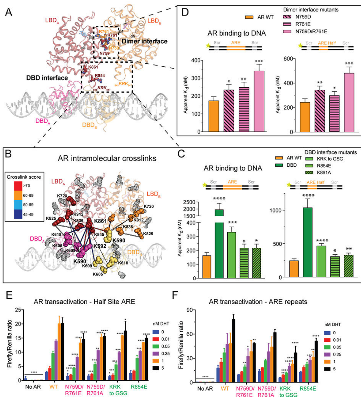
Figure 2. Structural basis for interdomain allostery.
