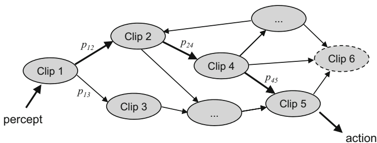
Fig. 1 Model of episodic and compositional memory (ECM) as a stochastic network of clips. Perceptual input, indicated by the bold arrow on the left , triggers a random motion through memory. The random motion between different clips is governed by transition weights (probabilities) that are continuously modified under the agent’s experience. p_{ij} denotes the probability of transition from Clip i to Clip j . If a sequence of transitions is taken that leads to a rewarded action (here illustrated by the sequence 1-2-4-5), the weights of all transitions involved in that sequence will be increased. Clips can also be modified and newly created (here indicated as Clip 6 with dashed boundary ) as part of the learning process. (Figure adapted from Briegel and De las Cuevas (2012).)
