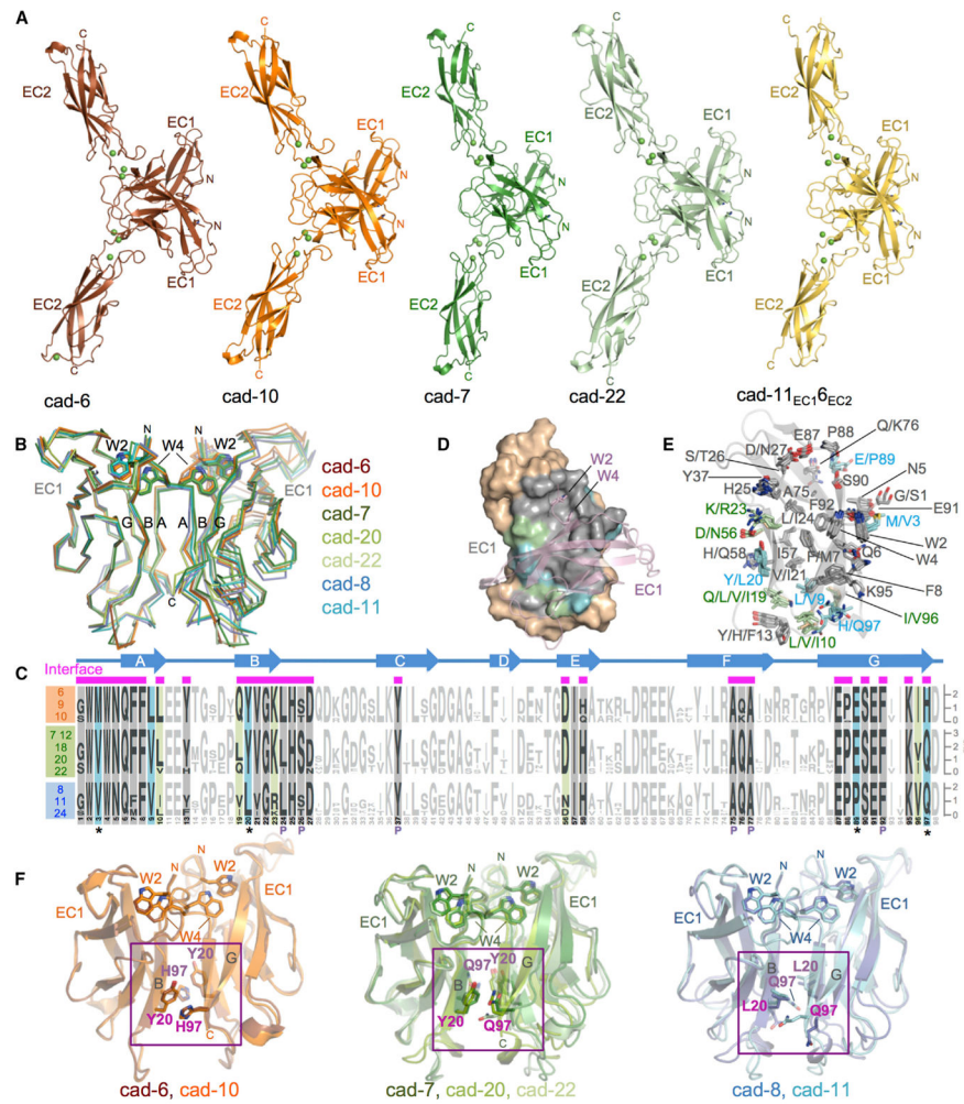
Figure 4. Crystal Structures of Type II Cadherin Homodimers and Analysis of Specificity Determinants
