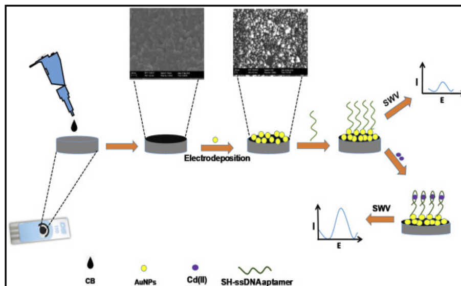
Fig. 10 Graphical demonstration of the procedure of fabrication and principle of detection of the \text{Cd}^{2+} using the aptasensor. This figure has been reproduced from ref. 169 with permission from Elsevier, copyright 2019.
