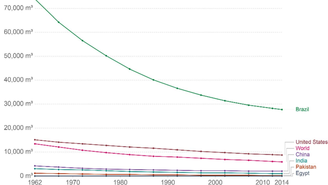
Fig. 2 Global freshwater demand and supply from 1962 to 2014. Long term freshwater use (a) and renewable freshwater resource per capita (b). This figure has been reproduced from ref. 16 with permission from World in Data, copyright 2017.
