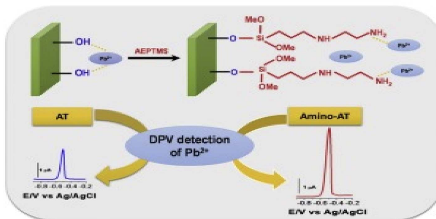
Fig. 19 Graphical summary illustrating the electrochemical detection of \text{Pb}^{2+} using the functionalized AAPTMS/GCE on DPV technique. This figure has been reproduced from ref. 208 with permission from Elsevier, copyright 2012.
