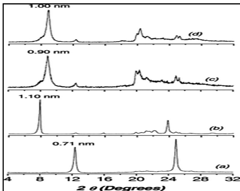
Fig. 18 XRD patterns of (a): K, (b): K–DMSO, (c): K–SiPCL and (d): K–SiPSH. This figure has been reproduced from ref. 207 with permission from WILEY-VCH, copyright 2011.
